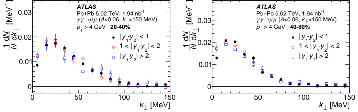
Figure 23: Dimuon k_{\perp} distributions in three intervals of |\Delta y| in the 20–40% (left) and 40–80% (right) centrality intervals, respectively. The distributions are self-normalized to allow the distributions to be directly compared. The error bars show combined statistical and systematic uncertainties.
