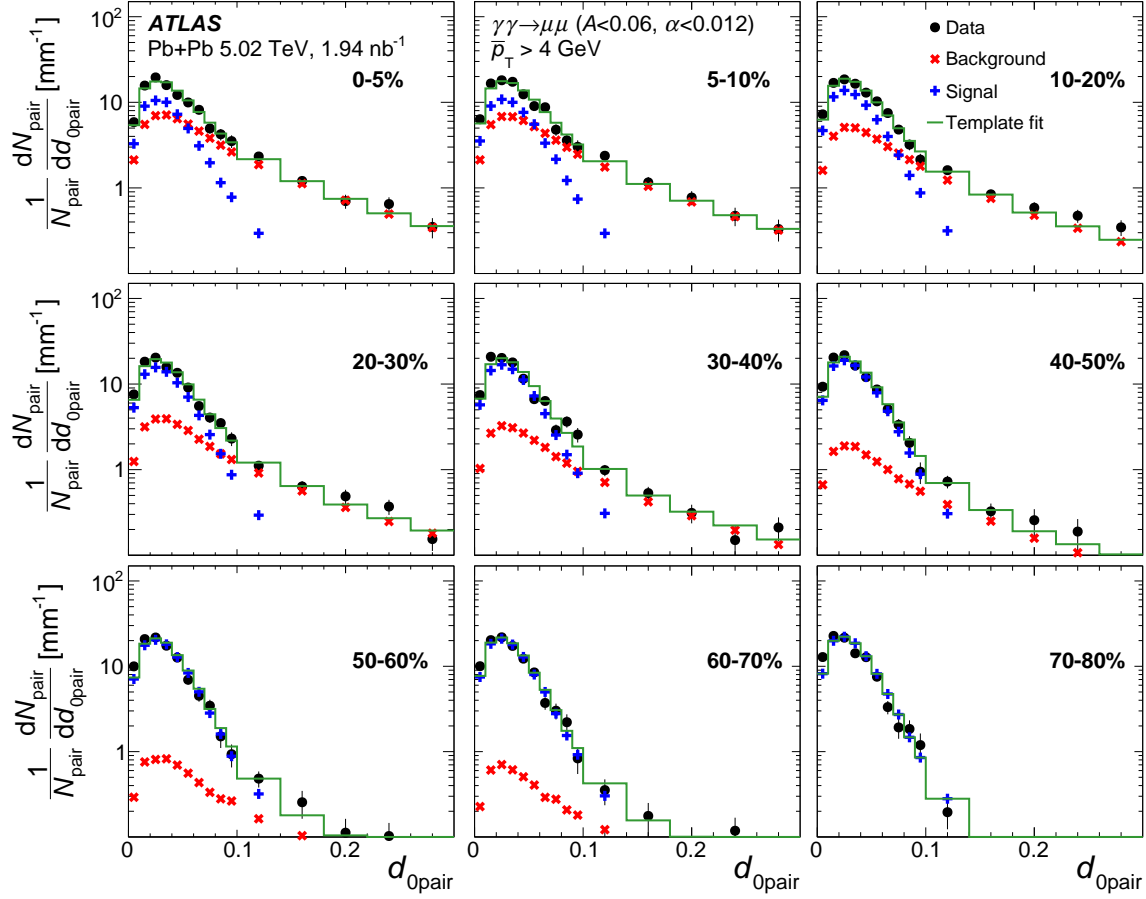
Figure 4: Results of template fits to measured d_{0\text{pair}} distributions for pairs passing the muon preselections, the (z_0 \sin \theta)_{\text{pair}} requirement and the Fid- \alpha selection ( A < 0.06 and \alpha < 0.012 ). Each panel represents a different centrality interval. The error bars shown on the data and the templates represent statistical uncertainties only. For many of the points, the error bars are smaller than the size of the marker.
