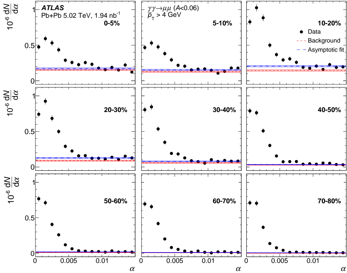
Figure 7: Measured \alpha distributions for pairs passing the full set of \gamma\gamma \rightarrow \mu^+\mu^- selections and in the Fid- \alpha region for nine centrality intervals. The error bars on the points indicate statistical uncertainties. Also shown are the background levels estimated from the d_{0\text{pair}} template fitting (red, fine-dashed lines) and from the asymptotic fits (blue, coarse-dashed lines). The widths of the lines indicates the statistical uncertainty of the background estimates.
