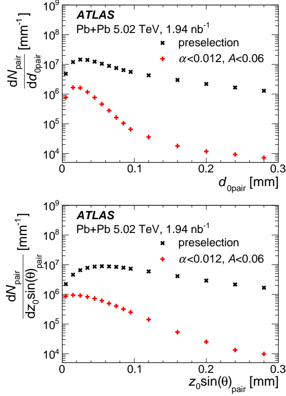
Figure 1: Distributions of d_{0\text{pair}} (top) and (z_0 \sin \theta)_{\text{pair}} (bottom) for muon pairs passing the preselections (black), and for pairs additionally passing the Fid- \alpha ( A < 0.06 , \alpha < 0.012 ) selection (red). The error bars in both panels correspond to the statistical uncertainties, and are typically too small to be seen. The pairs passing the Fid- \alpha selection have much smaller d_{0\text{pair}} and (z_0 \sin \theta)_{\text{pair}} values than pairs passing the preselections, due to the large HF background in preselected pairs.
