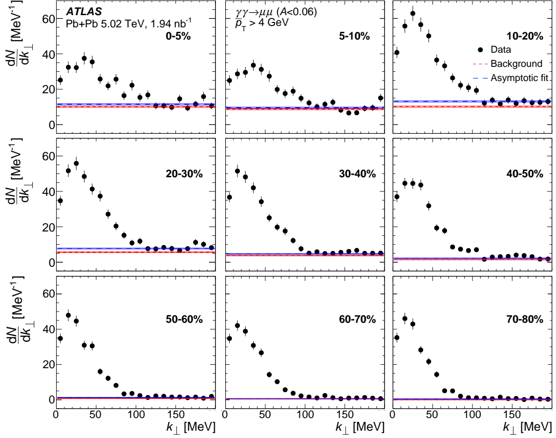
Figure 8: Measured k_{\perp} distributions for pairs passing the full set of \gamma\gamma \rightarrow \mu^+\mu^- selections and in the Fid- k_{\perp} region for nine centrality intervals. The error bars on the points indicate statistical uncertainties. Also shown are the background levels estimated from the d_{0\text{pair}} template fitting (red, fine-dashed lines) and from the asymptotic fits (blue, coarse-dashed lines). The widths of the lines indicates the statistical uncertainty of the background estimates.
