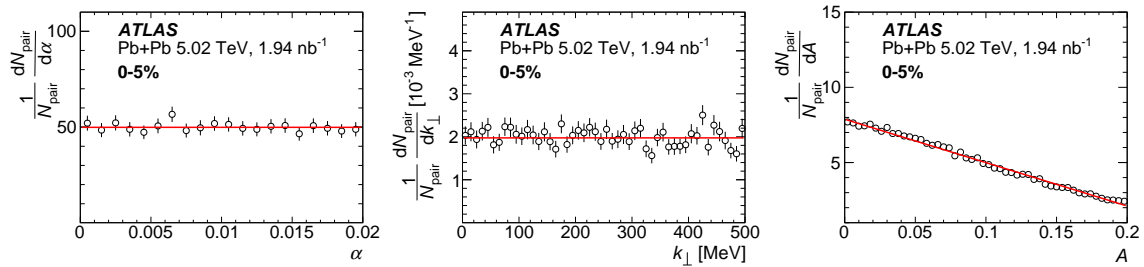
Figure 6: The heavy-flavor \alpha (left), k_{\perp} (middle), and A (right) distributions for the 0–5% centrality interval. The \alpha and k_{\perp} distributions are obtained by applying A > 0.06 to preselected pairs. The A distribution is obtained by applying \alpha > 0.012 . The error bars correspond to statistical uncertainties. The lines indicate fits to constant functions for \alpha and k_{\perp} and to a linear function for A .
