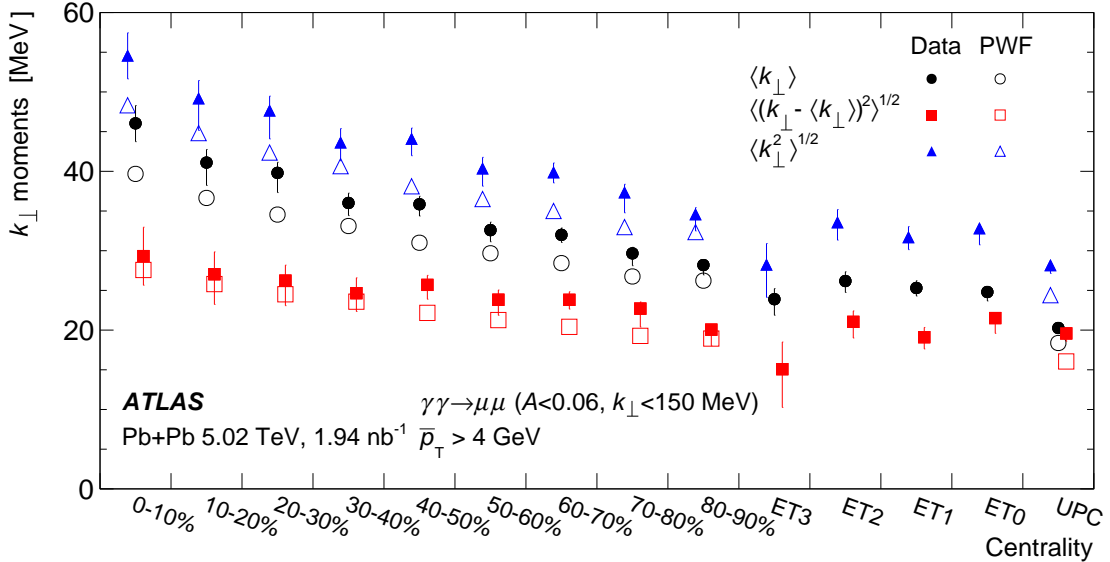
Figure 21: Moments of the \gamma\gamma \rightarrow \mu^+\mu^- k_{\perp} distributions as a function of centrality compared with the PWF predictions. The error bars indicate combined statistical and systematic uncertainties. In some bins, the statistical uncertainties, determined both by the number of counts and by their k_{\perp} distribution, dominate.
