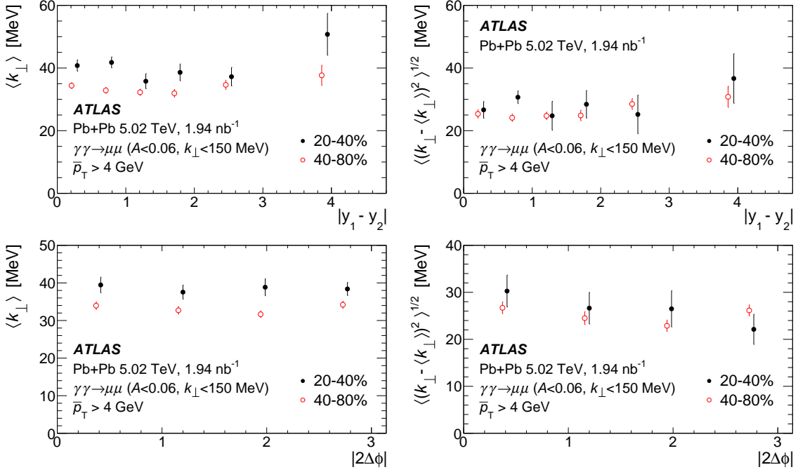
Figure 25: The average (left) and the standard deviation (right) of the \gamma\gamma \rightarrow \mu^+\mu^- k_{\perp} distributions in the 20–40% and 40–80% centrality intervals as a function of |\Delta y| (top) and |2\Delta\phi| (bottom). Results are shown for |\Delta y| intervals of width 0.5 for |\Delta y| < 2.0 , and two additional intervals covering 2.0 \leq |\Delta y| < 3.0 and 3.0 \leq |\Delta y| < 4.8 . The |2\Delta\phi| results are shown for four equal intervals covering [0, \pi] . The error bars show combined statistical and systematic uncertainties. The points are staggered for clarity of presentation.
