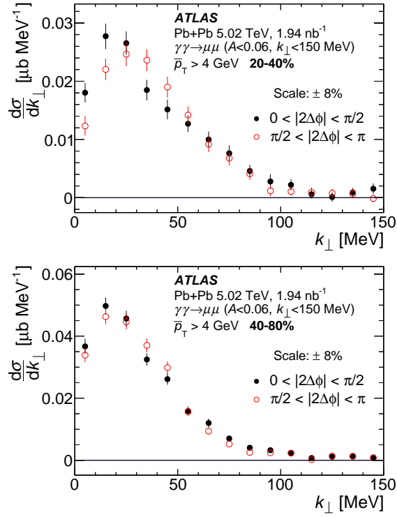
Figure 24: Differential cross-sections for \gamma\gamma \rightarrow \mu^+\mu^- production as a function of k_{\perp} for two intervals of |2\Delta\phi| : 0 < |2\Delta\phi| < \pi/2 and \pi/2 < |2\Delta\phi| < \pi in the 20–40% (top) and 40–80% (bottom) centrality intervals, respectively. The error bars show combined statistical and systematic uncertainties.
