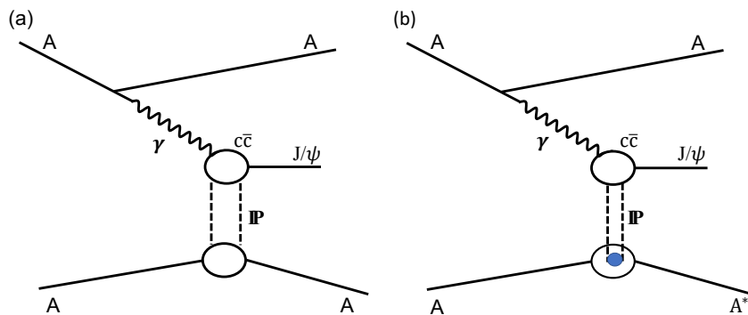
Figure 1. Schematic diagrams for charmonium production in (a) coherent and (b) incoherent UPC heavy-ion collisions. For incoherent production, the pomeron is emitted from a single nucleon, indicated by the blue dot, and the nucleus typically dissociates, indicated by A^* .
