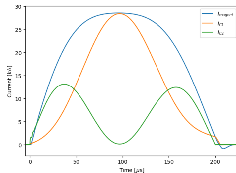
Figure 3: Current pulse through the magnet produced by the circuit described in Fig. 2. Also shown are the current outputs from the two capacitor banks.
