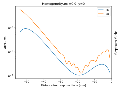
Figure 7: \frac{\Delta B}{B_0} and \frac{\Delta B dl}{B_0} homogeneity for LHC beam along the midplane for 2D and 3D simulations.
