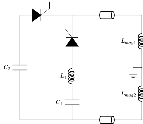
Figure 2: Conceptual circuit diagram.
