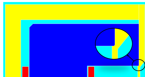
Figure 1: Top half cross-section of proposed magnet with zoom of the inset feature.
