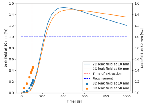
Figure 5: Leak field at 10 mm and 50 mm from the septum blade for 2D and 3D simulations.
