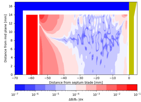
Figure 6: 3D simulation homogeneity \frac{\Delta B dl}{B_0} for LHC beam.
