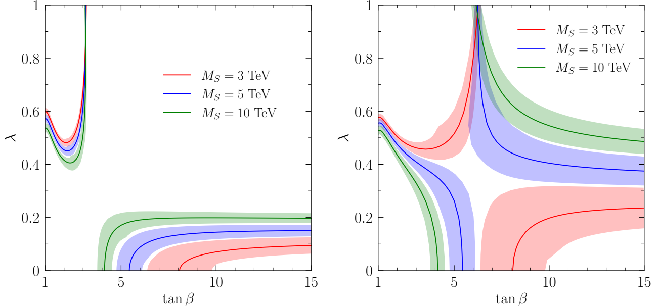
Figure 2: Regions of the \tan\beta - \lambda plane that yield M_h = 125.25 GeV, for \kappa = \lambda (left) or \kappa = 2\lambda (right), in the NMSSM scenario described in the text. The three sets of lines in each plot correspond to different values of the common mass term for the third-generation sfermions. The band around each line is our estimate of the theory uncertainty.
