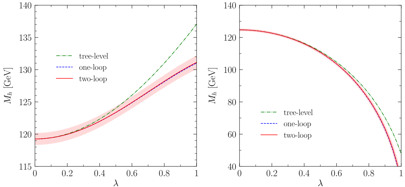
Figure 1: Higgs-mass prediction as a function of \lambda , for \tan\beta = 3 (left) or \tan\beta = 5 (right), in the NMSSM scenario described in the text. The three lines in each plot correspond to different accuracies of the NMSSM-specific contribution to the matching condition for \lambda_{\text{SM}} . The band around the red, solid line is our estimate of the theory uncertainty.
