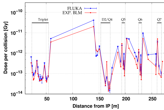
Figure 4: BLM pattern along the LSS on the right side of IP1, as measured during the Pb-Pb physics fill #7473 in 2018 and simulated with FLUKA. Experimental doses are divided by the product of the fill luminosity and the 438 b cross section value, corresponding to the sum of the INI and EMD cross sections.
