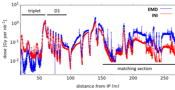
Figure 1: Dose profile below the beam line along the LSS on the right of IP1 as induced by Pb-Pb collisions. Values are averaged over a 40 cm horizontal interval centred on the machine axis and a 20 cm vertical interval centred 60 cm below the machine axis. They are normalized to a reference integrated luminosity of 1 \text{ nb}^{-1} . INI and EMD contributions are shown separately.
