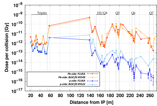
Figure 3: BLM pattern along the LSS on the right side of IP1, as measured during the indicated Pb-p (orange) and p-Pb (light blue) physics fills and simulated with FLUKA (red and blue, respectively). Experimental doses are divided by the product of the fill luminosity and the 2.11 \text{ b} INI cross section value.
