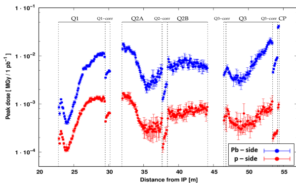
Figure 2: Peak dose profile in the inner coils of the triplet as a function of the distance from the IP, induced by Pb-p collisions on the Pb-side (blue) and the p-side (red). Values are normalized to a reference integrated luminosity of 1 \text{ pb}^{-1} .
