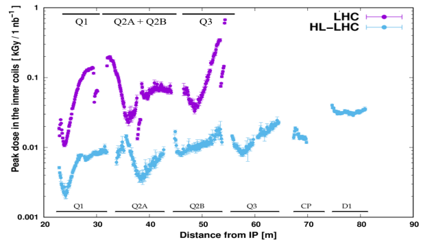
Figure 5: Peak dose profile in the inner coils of the LHC Q1-Q3 string (purple) and HL-LHC Q1-D1 string (blue), as induced by INI and EMD events in Pb-Pb collisions. For the purpose of comparison, values are normalised in both cases to a reference integrated luminosity of 1 \text{ nb}^{-1} .
