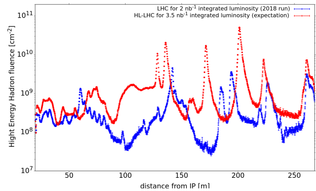
Figure 6: High energy hadron fluence profile along the LSS on the right of IP1 as induced by Pb-Pb collisions in the HL-LHC (red) and LHC (blue) configuration. Values averaged over a 40 cm horizontal interval centred on the machine axis and a 20 cm vertical interval centred 30 cm from the floor level. They are normalized to an annual integrated luminosity of 3.5 \text{ nb}^{-1} and 2 \text{ nb}^{-1} , respectively. INI and EMD contributions are added up according to their cross sections.
