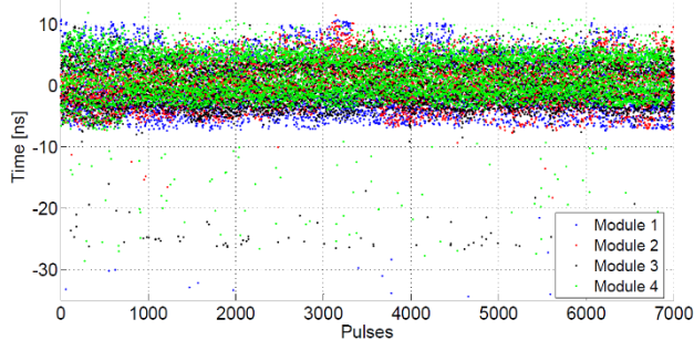
Figure 6: Jitter measurement of all KFA45 modules during operation at 54 kV in 2017.
