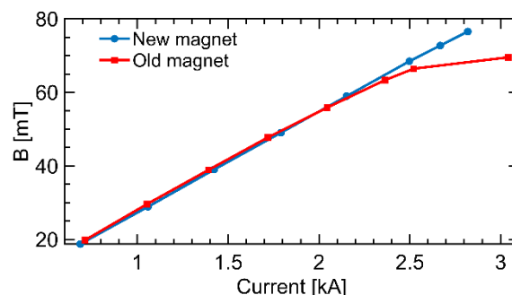
Figure 1: Measured saturation of the old (red) and new (blue) magnet.
