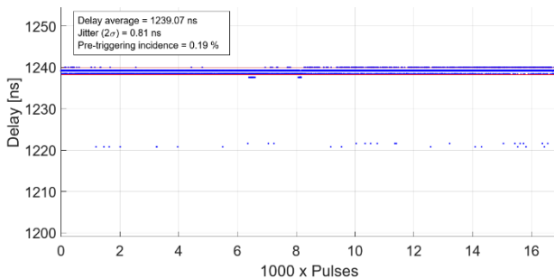
Figure 7: Jitter measurement on one module of the new MS triggering system pulsing at 60 kV.
