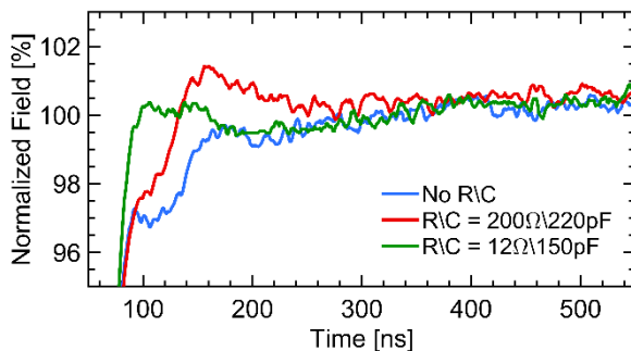
Figure 4: Measured field of the new magnet with different RC filters attached to the CB.
