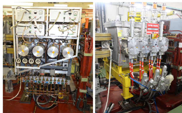
Figure 2: The old KFA45 magnet in the tunnel with s/c thyatron, TMR and oil cooling (left) and the new redesigned KFA45 in s/c configuration with the new SF6 gas free transmission cables (red) and a FC-77 filled connection box (right).
