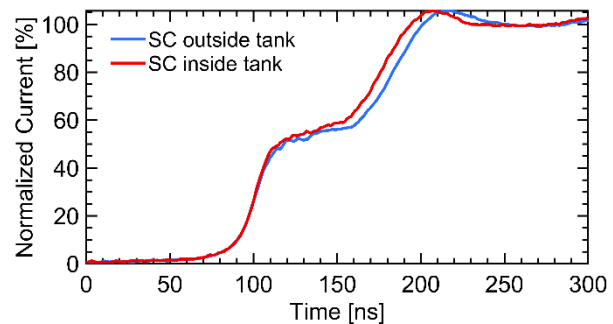
Figure 5: Measured current rise time of the new magnet with the s/c termination in the CB (blue) and directly at the module (red).
