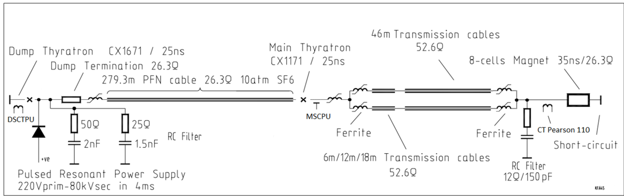
Figure 3: Schematic of the PS injection kicker system as installed with modified MS ferrites, dephasing cables, new Tx-cables, magnet CB ferrites and magnet CB filters.
