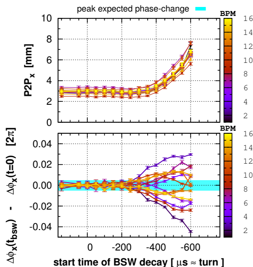
Figure 4: Change to horizontal inter-BPM phase advance ( \Delta\phi_x ) measured for different start time of BSW decay, with respect to value at nominal timing ( \Delta\phi_x(t=0) ).
