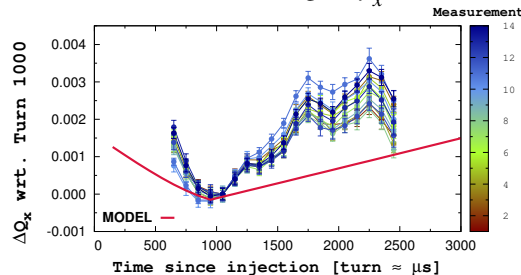
Figure 5: \Delta Q_x (w.r.t. Q_x after 1000 turns) vs time since injection. Data points are measurement for each injection. Errors are RMS over 16 BPMs for each measurement.
