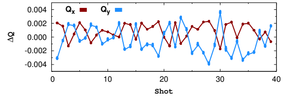
Figure 10: Example of cycle-to-cycle variation of Q_{x,y} .
