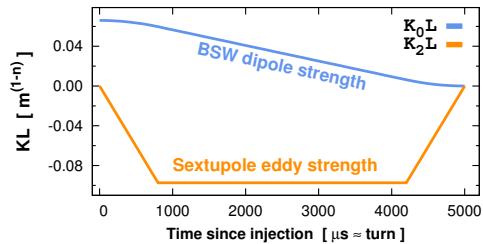
Figure 2: Integrated dipole and sextupole strength during collapse of injection (BSW) orbit bump.
