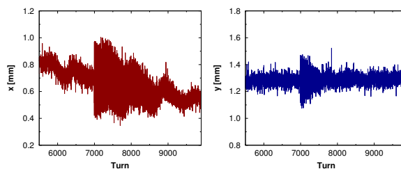
Figure 6: Example of TbT data at 160 MeV with Q_{x,y} = 4.40, 4.45 and maximum powering of the Q -kicker.
