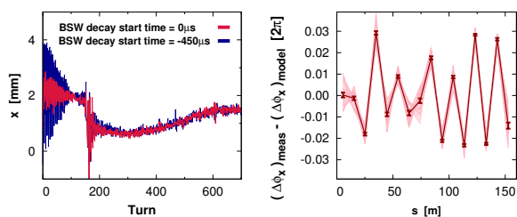
Figure 3: Left: example of injection oscillations for nominal timing of the BSW decay (red) and with the start time of the BSW decay shifted forwards by 450 s (blue). Right: phase-beating with respect to nominal PSB model measured from injection oscillations, shaded area indicates the range of phase-beat measured over 20 injections at Q_x = 4.40 .
