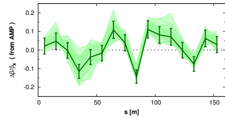
Figure 9: Measured \beta -beat from amplitude under optimal conditions with the Q-kicker. Error-bars are combination of std. over 30 injections together with uncertainty on reconstruction from error on action measurement. Shaded area indicates range of \beta -beat measured over 30 injections.
