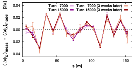
Figure 7: Reproducibility of horizontal phase-beat at flat-bottom turn 7000 and turn 15000 over 3 week period.
