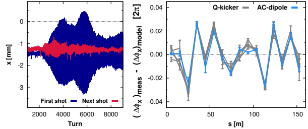
Figure 11: Left: TbT data for 2 consecutive shots with same AC-dipole excitation. Right: comparison of phase-beat at flat-bottom measured with Q-kicker and AC-dipole.
