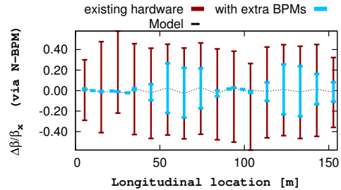
Figure 1: \beta -beat via N-BPM method for ideal tracking simulations with existing PSB BPMs (red), and with extra BPMs (blue) at optimal \Delta\phi in periods 1, 2, 3, 10 and 11. Error bars are the systematic uncertainty on the reconstruction.
