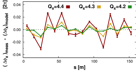
Figure 8: Dependence of horizontal phase-beat on working point at flat-bottom turn 15000.
