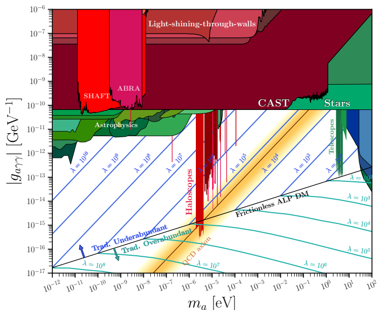
Figure 1. Axion coupling to photons g_{a\gamma\gamma} \sim \alpha/(2\pi f_a) versus its mass for the case where the axion couples to two separate non-abelian gauge groups as studied in section 5. The presence of friction can open up the ALP-dark-matter parameter space: for different values of the enhancement parameter \lambda , the correct ALP DM relic density is obtained for the traditionally underabundant region along the blue lines and for the traditionally overabundant region along the cyan lines (assuming \alpha_{\text{thr}} = 0.1 and g_{\rho,s} \sim \mathcal{O}(10) , see section 5 for details). Experimental bounds adapted from AxionLimits [23].
