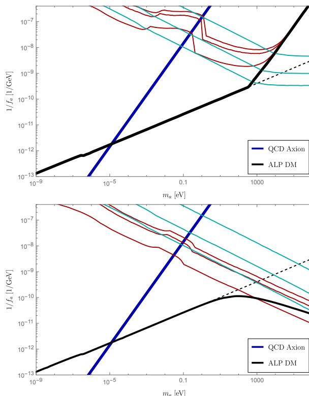
Figure 3. Predictions for the values of \{m_a, 1/f_a\} that reproduce the correct axion DM relic density (black solid lines), taking into account thermal friction for \alpha_{\text{thr}} = 0.2 ( top panel ) and \alpha_{\text{thr}} = 0.4 ( bottom panel ). They deviate with respect to the standard frictionless computation, which is shown in dashed black lines. The red lines are constant depletion factor e^{-D} , with D defined in eq. (3.15) and correspond to 10^{-20} , 10^{-10} , 10^{-1} from top to bottom. The cyan lines are lines of constant enhancement factor (m_{\text{osc}}/4H_{\text{osc}})^{3/2} and correspond to 100, 10, 2 respectively from top to bottom.
