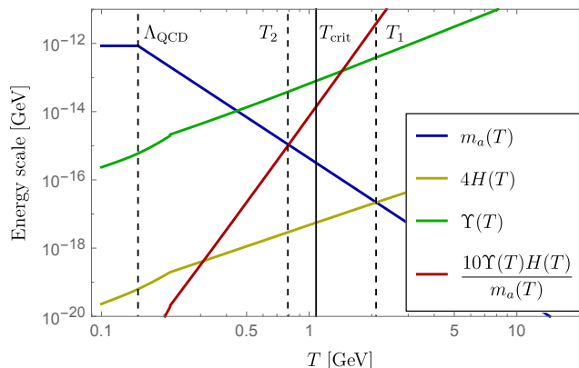
Figure 5. An example of the scenario that could open up the parameter space for QCD axion dark matter. The vertical lines represent the relevant scales defined in eq. (5.5) except for \Lambda which is too low to be seen in the panel. Normally the onset of oscillations occurs at T_1 , however the friction can delay the onset at most until T_2 . If the dark sector spontaneously breaks at T_{\text{crit}} then the correct abundance is obtained. For this example we used f_a = 10^{10} GeV, \lambda = 10^5 and \Lambda = 10^{-3} GeV.
