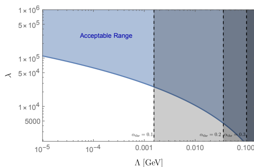
Figure 6. Region of the parameter space \{\lambda, \Lambda\} that allows to reproduce the correct axion DM relic density. The blue shaded region ensures that the QCD axion does not roll until T_{\text{crit}} at which time the dark sector is spontaneously broken. Finally the gray shaded regions signal the parameter space for which our expressions for the thermal friction breakdown before T_{\text{crit}} is reached for different options of the threshold value of the running coupling.
