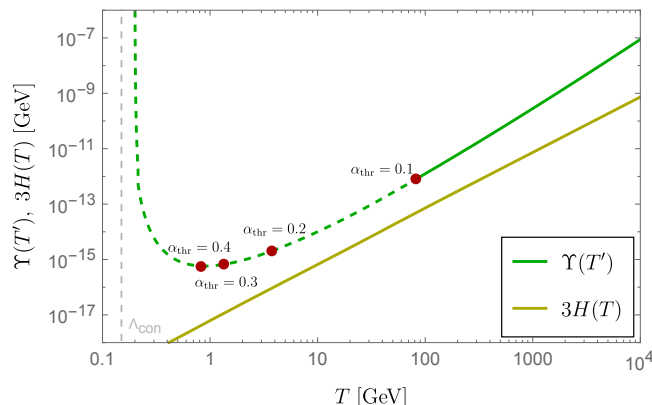
Figure 4. Gauge friction versus Hubble friction for some example parameter values. The red dots denote the instant we switch off the friction effects depending on the largest acceptable value of the gauge coupling \alpha_{\text{thr}} .
