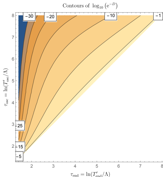
Figure 2. Contour plot of the overall suppression factor e^{-D} where D given by eq. (3.16) for f = 10^8 GeV and \Lambda = 150 MeV.
