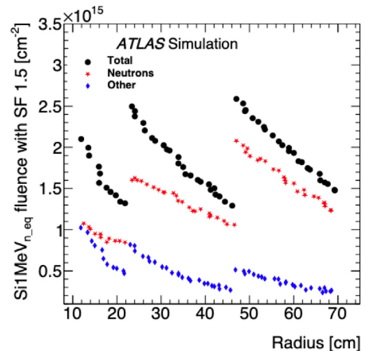
Fig. 3. Maximum fluence the modules will have to face in their Lifetime as a function of the radial position in the detector. The three regions reflect the different replacement scenarios (every 1/fb for the inner ring, every 2/fb for the middle ring, while the outer ring will not be replaced).
