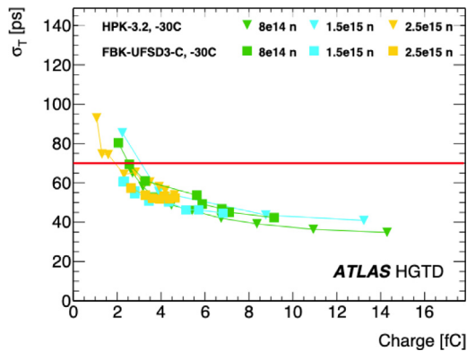
Fig. 6. Time resolution as a function of the collected charge for neutron irradiated LGADs from different producers (HPK, FBK) with a 50 \mu\text{m} active thickness. These measurements have been made at -30^\circ\text{C} , in the laboratory with a \beta source using a custom electronics read-out board. The typical error bar is about 3 ps. The red line shows that in these conditions better than 70 ps time resolution is obtained at 4 fC. Source: Figure taken from Ref. [3].
