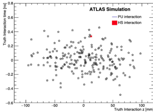
Fig. 1. Visualization of the truth interactions in a single bunch crossing in the z-t plane, showing the simulated Hard Scatter (HS) t\bar{t} event interaction (red) with pile-up interactions superimposed (black) for \langle\mu\rangle = 200 .
