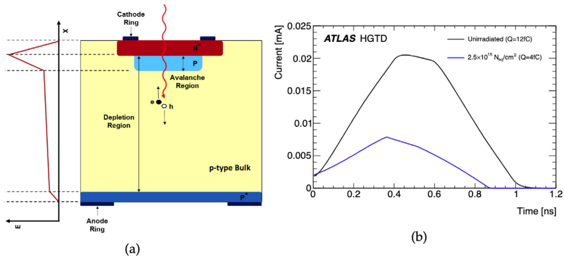
Fig. 5. Cross section of an LGAD (a) and simulated signal current in LGADs at start and after full integrated neutron fluence (b). Source: From Ref. [3].
