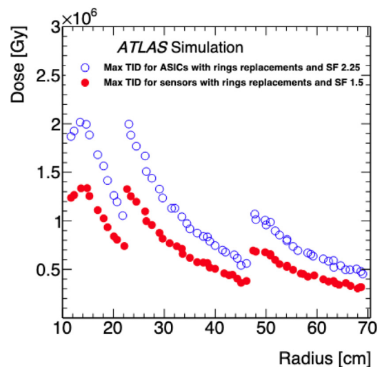
Fig. 4. Ionizing dose for HL-LHC with scale factor applied and considering replacements.
