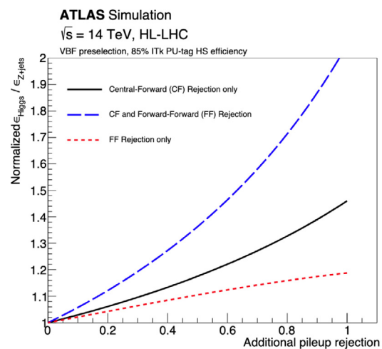
Fig. 8. Normalized signal over background gain relative to ITk-only pile-up jet suppression performance, as a function of the additional pile-up jet rejection from HGTD. The solid black (dotted red) line represents the HGTD improvement from the Central-Forward (Forward-Forward) event topologies separately. The dotted blue line shows the total improvement when the combined HGTD+ITk pile-up suppression algorithm is applied to all jets in the event.
