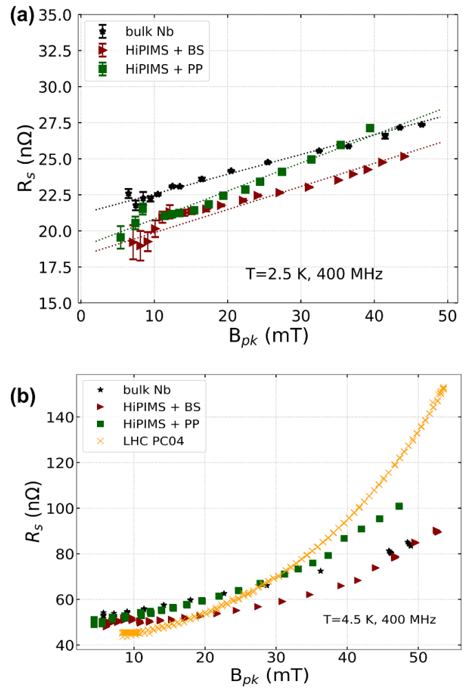
Figure 6. Surface resistance R_s as a function of the peak magnetic RF field B_{pk} at f_0 = 400 MHz, T = 2.5 K (a) and T = 4.5 K (b) for the three characterized samples: bulk niobium (black stars), HiPIMS + BS coating (red triangles), HiPIMS + PP coating (green squares) and LHC PCO4 cavity (orange crosses). The dashed straight lines in (a) represent the best linear fit of the experimental data.
