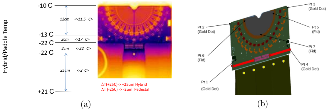
Figure 4: Temperature gradient along the silicon and the hybrid due to the to isothermal effect, in the case of a cooling temperature at -25^{\circ}\text{C} (a). A drawing of the VELO module illustrating the approximate positions of the survey points (b).
