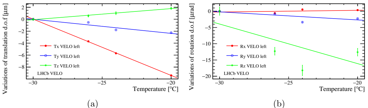
Figure 5: Variations of translation (a) and rotation (b) d.o.f of the left VELO, calculated when two halves and modules alignment is performed. The dashed grey line in the left plot is the min variation needed for an update in T_x .
