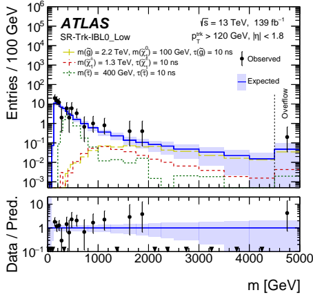
(a) SR-Trk_IBL0_Low
