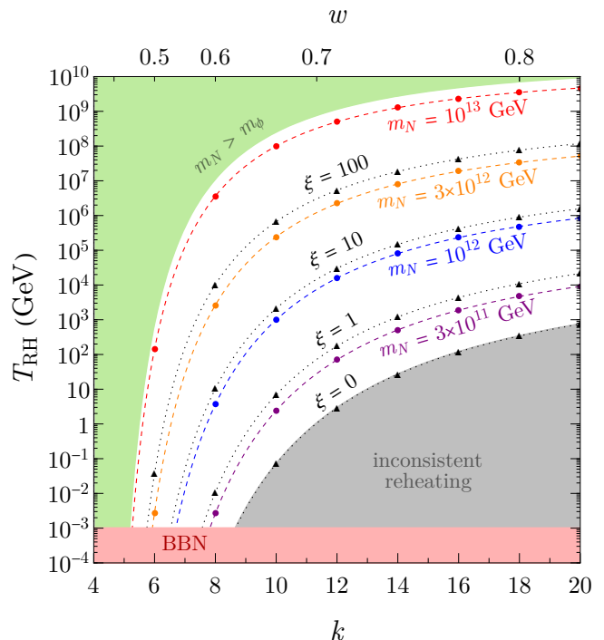
FIG. 2. The colored dashed curves show values of the reheating temperature T_{\text{RH}} required to explain the observed baryon asymmetry as a function of k , the exponent of the potential defined in Eq. (4), for different choices of the right-handed neutrino mass m_N . The black dotted lines show the reheating temperature obtained from purely gravitational reheating for different choices of \xi , the non-minimal gravitational coupling constant defined in Eq. (20). A minimal gravitational coupling ( \xi = 0 ) gives a minimum T_{\text{RH}} , excluding the gray region. The upper x-axis labels the equation of state w = (k-2)/(k+2) of the inflaton, during reheating.
