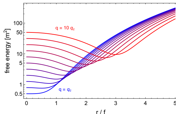
Figure 1. Free energy (2.7) for different values of the total charge q , leading to a finite vev for the AD field for q above the critical value q_c . For thermal corrections, see section 3.
