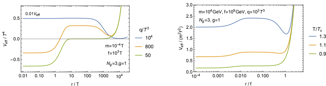
Figure 3. Effective potential including thermal contributions for the case with charge transfer to the axion as a function of the radius of the AD field r for several total charges q .
