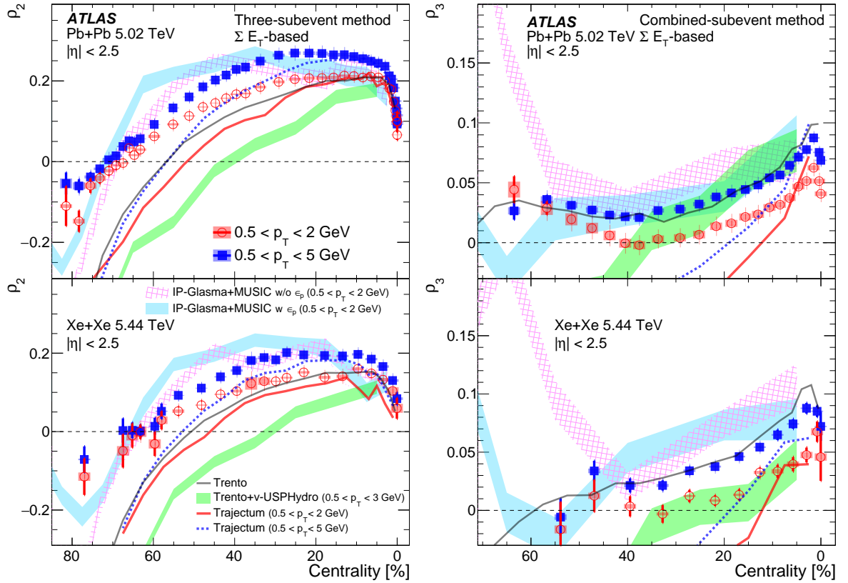
Figure 7: The \rho_2 (left) and \rho_3 (right) values in Pb+Pb (top) and Xe+Xe (bottom) collisions in two p_T ranges and |\eta| < 2.5 compared with various models: Trento [74] and Trajectum [75] models in solid lines and v-USPhydro [24] and IP-Glasma+MUSIC [26] hydrodynamic models in shaded bands, which represent the statistical uncertainties of the model calculations.
