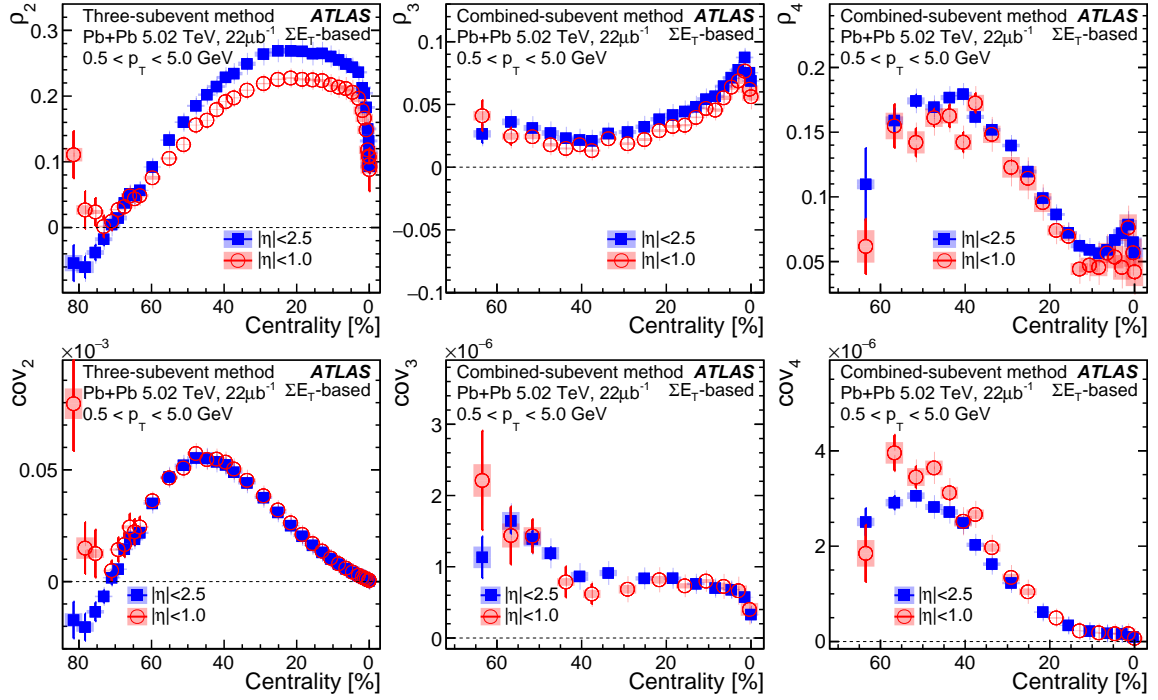
Figure 4: The centrality dependence of \rho_n (top) and \text{cov}_n (bottom) for n=2 (left), 3 (middle), and 4 (right) in Pb+Pb collisions compared between the two choices for the \eta ranges from Table 1. They are calculated using the event-averaging procedure based on \Sigma E_T . The error bars and shaded boxes represent statistical and systematic uncertainties, respectively.
