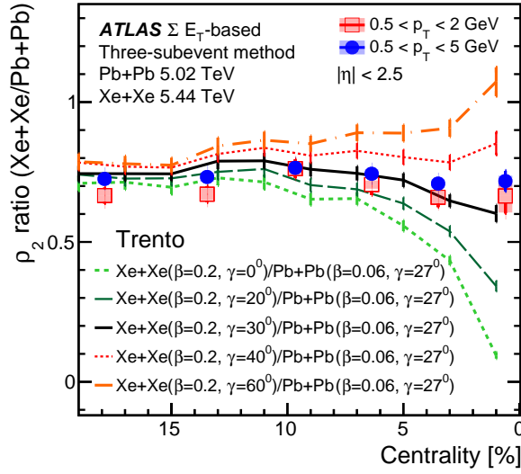
Figure 9: Comparison of \rho_2 ratios, \rho_{2,Xe+Xe}/\rho_{2,Pb+Pb} , with the Trento model for various quadrupole deformation parameter values [31] in two p_T ranges. The Trento model results are connected by lines for better visualization.
