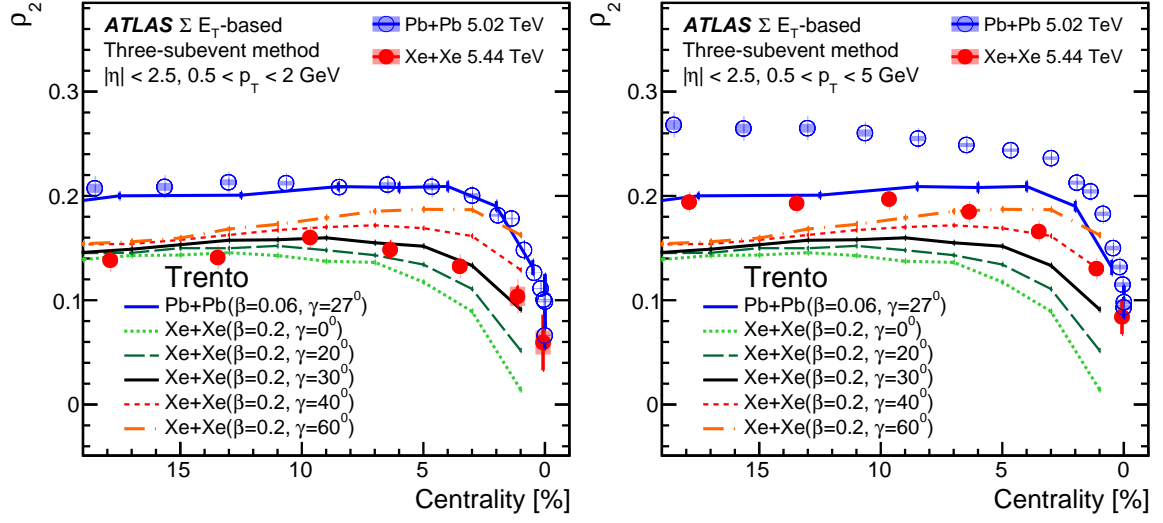
Figure 8: Comparison of \rho_2 in Xe+Xe and Pb+Pb collisions with the Trento model for various quadrupole deformation parameter values [31] in 0.5 < p_T < 2 GeV (left) and 0.5 < p_T < 5 GeV (right) as a function of centrality. The same Trento results are used in both panels, and they are connected by lines for better visualization.
