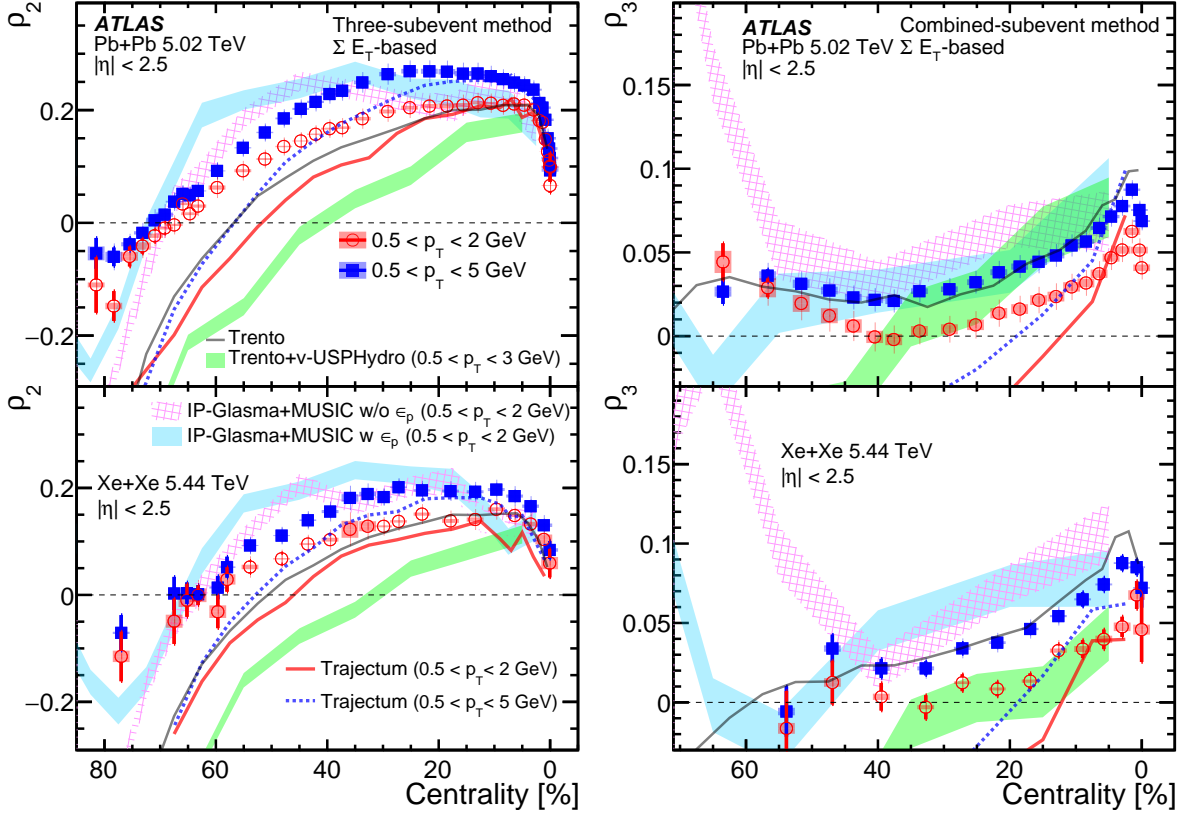
Figure 7: The \rho_2 (left) and \rho_3 (right) values in Pb+Pb (top) and Xe+Xe (bottom) collisions in two p_T ranges and |\eta| < 2.5 compared with various models: Trento [76] and Trajectum [77] models in solid lines and v-USPhydro [26] and IP-Glasma+MUSIC [22] hydrodynamic models in shaded bands, which represent the statistical uncertainties of the model calculations.
