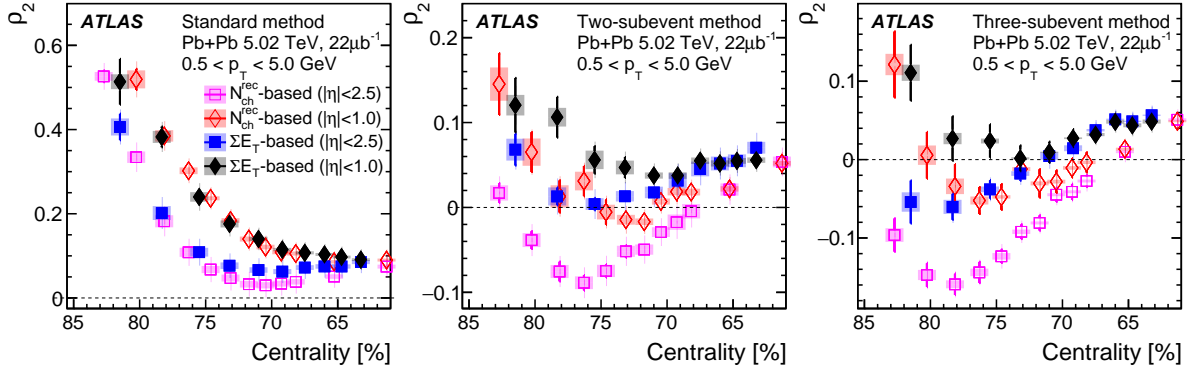
Figure 6: The centrality dependence of \rho_2 in Pb+Pb collisions in the peripheral region of 60–84% for the standard method (left), two-subevent method (middle) and three-subevent method (right), compared between the N_{\text{ch}}^{\text{rec}} -based and \Sigma E_T -based event-averaging procedures and two \eta ranges. The error bars and shaded boxes represent statistical and systematic uncertainties, respectively.
