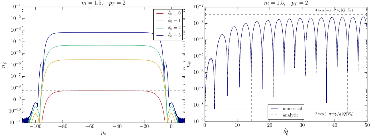
Figure 1: Numerical solutions for the total number of produced particles after turning off the background fields. Left : spectrum of produced particles for different values of the background axion velocity \dot{\theta}_0 as a function of the fermion momentum p_z . The gray dashed line corresponds to the standard Schwinger effect formula, n_\psi = 2 \exp(-\pi m_T^2/g|Q|E_0) , where the factor 2 accounts for the chirality. Right : the height of the spectrum (at p_z = -50\sqrt{g|Q|E_0} ) as a function of \dot{\theta}_0^2 . The blue line corresponds to the numerical solution of the time evolution equation of the Bogoliubov coefficients, while the gray dashed line shows the analytical expression (2.17). In both figures, we take m = 1.5 and p_T = 2 in units of g|Q|E_0 = 1 .
