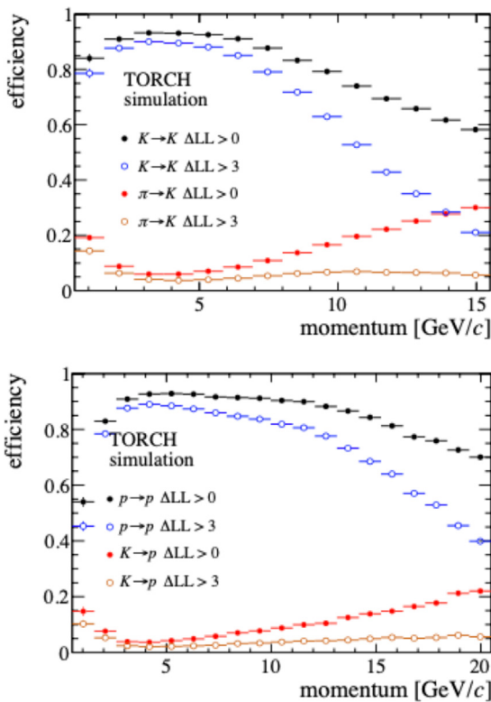
Fig. 5. TORCH PID performance in LHCb in HL-LHC data taking conditions. Two different likelihood requirements are shown for kaon-pion separation efficiency (top) and for proton-kaon separation efficiency (bottom).
