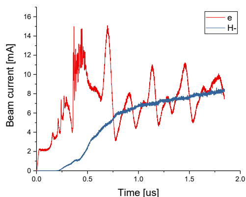
Figure 5: Time evolution of the extracted H^- current (blue line) and co-extracted electron (red line) current for the IS03 PE45 system simulated with ONIX using a 10 kV extraction voltage. H^- originates from volume and plasma surface production modes and e^-/H^- current ratio tends to 1.
