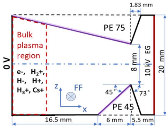
Figure 2: Schematic view of the simulation domains used in the ONIX code ( x - z mid plane) for modelling beam formation of IS03b PE45 bottom and PE75 top. The filter field (FF) orientation is indicated. The PE bore diameter is 8 mm.
