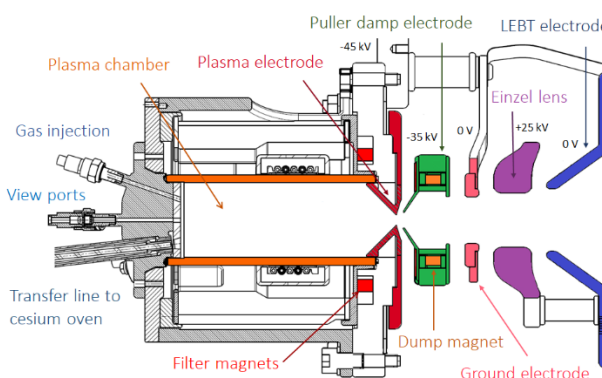
Figure 1: IS03b Linac4 H - ion source and extraction system. This source operates in volume and plasma surface H - production modes.
