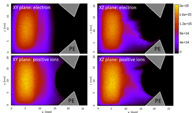
Figure 4: Density maps of electron (top) and positively charged particles ( H^+ , H_2^+ , H_3^+ ) (bottom) in the ( x - y ) (left) plane and ( x - z ) (right) plane where filter field generated asymmetry is clearly visible.
