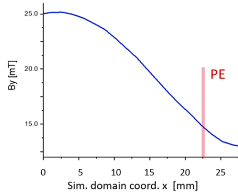
Figure 3: Magnetic field strength along beam-axis ( x ). The red line indicates the location of the plasma electrode (PE) aperture centred.
