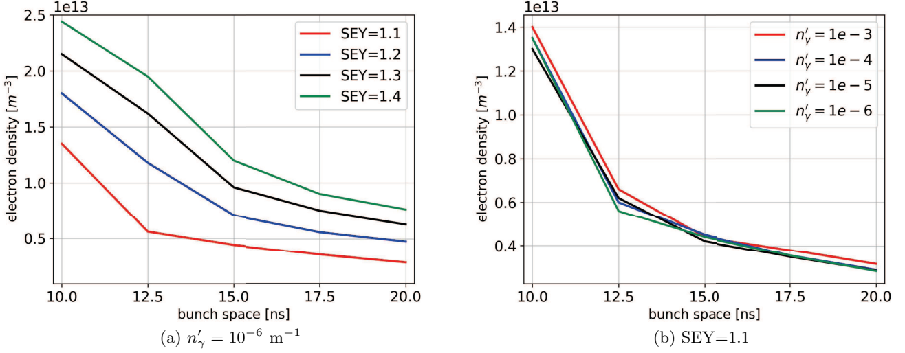
Fig. 5: Maximum central electron density for the Furman-Pivi model as a function of bunch spacing, varying either the SEY yield (left) or the photoelectron emission rate (right).
