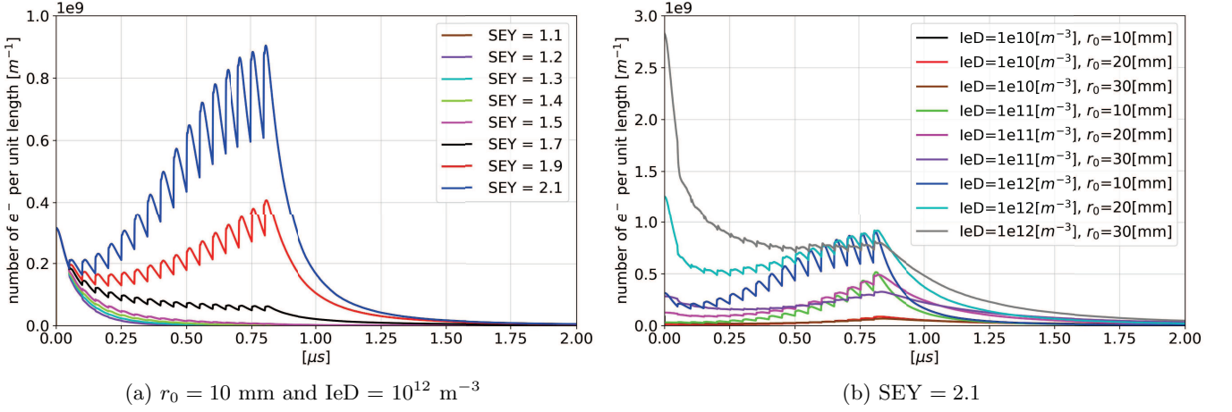
Fig. 2: Simulated electron-cloud evolution from an initial uniform seed for DR injection, using the Furman-Pivi model. 16 bunches with 50 ns spacing are followed by a gap.
