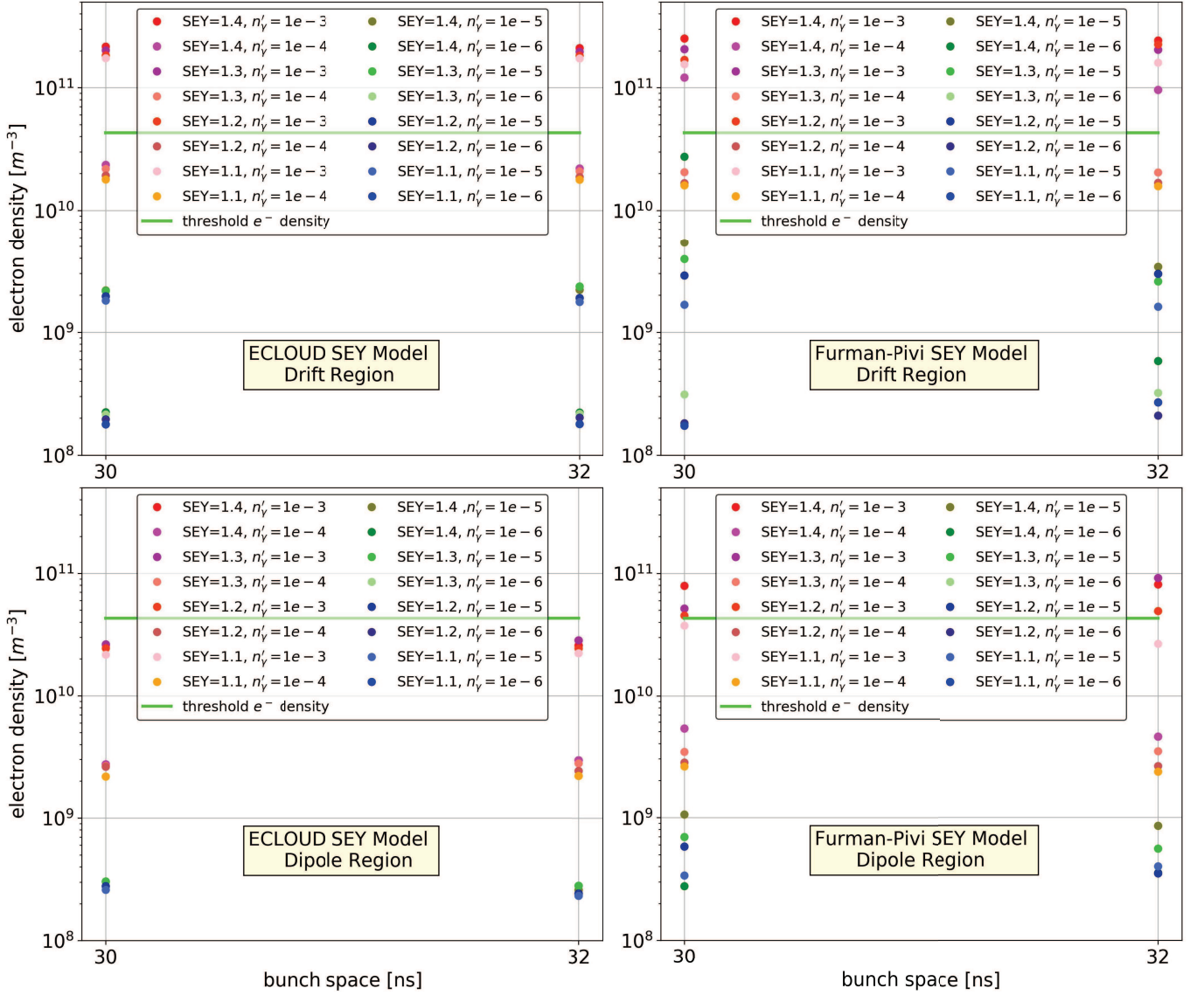
Fig. 8: Simulated electron densities at the center of the beam pipe for the FCC-ee arc dipole & drift regions using the new baseline beam parameters for four IPs [21]
