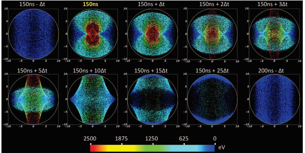
Fig. 3: Kinetic energy distributions of electrons inside the wiggler magnet chamber at particular time steps between two bunch arrivals as indicated (with \Delta t = 62.5 \text{ ps} ). for FCC-ee DR extraction.
