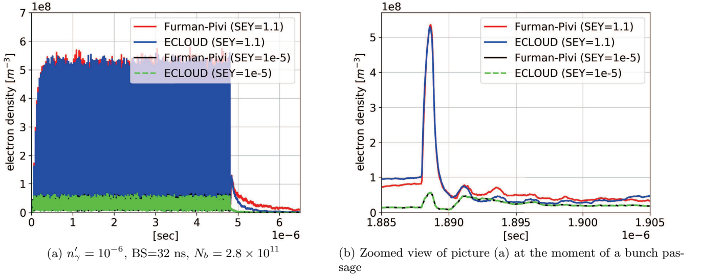
Fig. 6: Minimum central electron cloud density versus time, comparing SEY models and defining the reference electron formation level for SEY \approx 0 .
