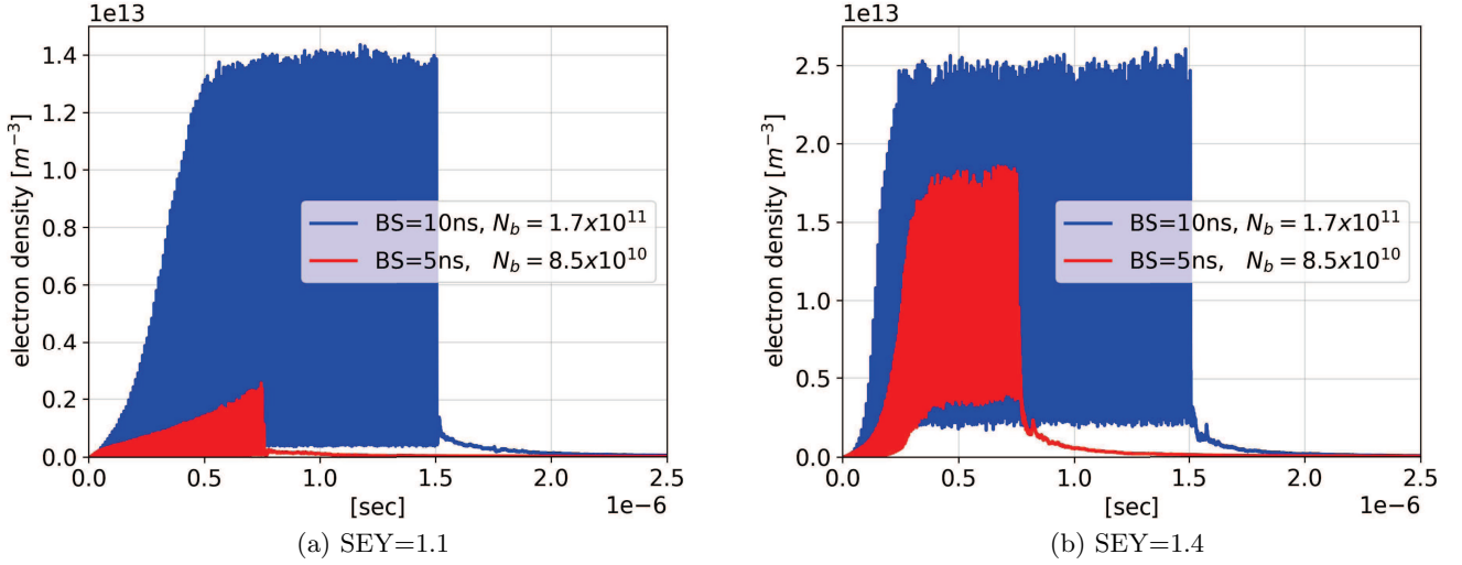
Fig. 7: Time evolution of the central electron density for bunch spacings of 10 and 5 ns, with associated bunch population N_b = 1.7 \times 10^{11} \text{ m}^{-3} and 8.5 \times 10^{10} \text{ m}^{-3} , respectively, at a high electron generation rate of n'_\gamma = 10^{-3} \text{ m}^{-1} (BS:bunch spacing, N_b : bunch population)
