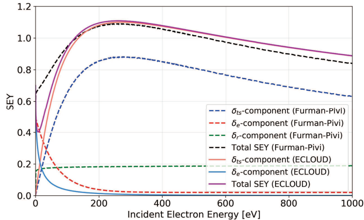
Fig. 1: Composition and overall shape for the two SEY models.
