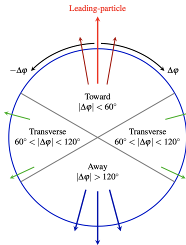
Figure 1: Illustration of the toward, transverse, and away regions in the azimuthal plane with respect to the leading particle direction. The figure has been taken from Ref. [14].
