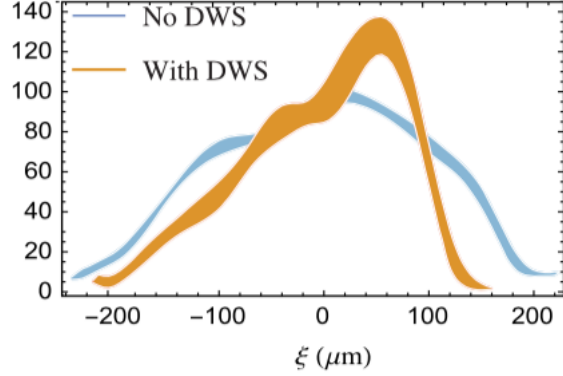
Figure 6. Ramped current profile generated from wakefield modulation compared to unperturbed beam. Adapted from [74].
