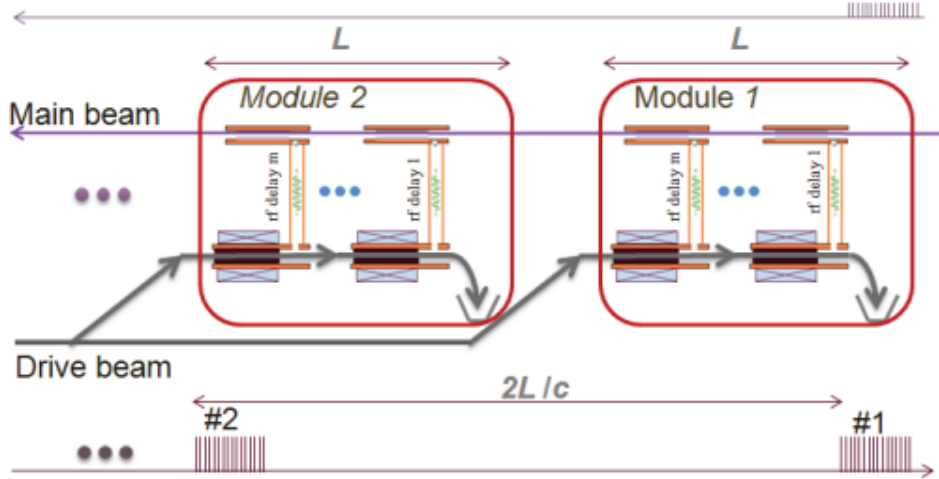
Figure 10. Schematic of TBA in two stages. (Reused from Ref. [83]).
