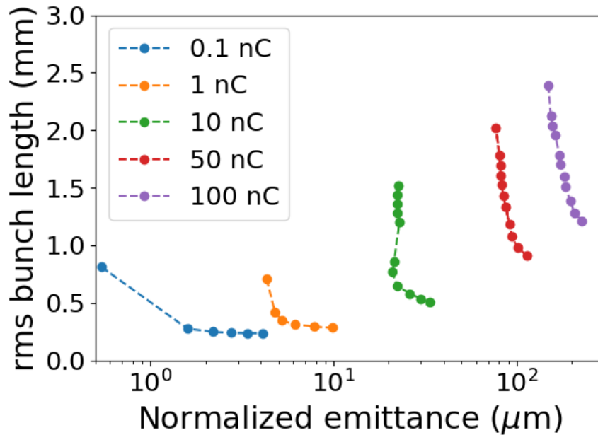
Figure 2. AWA L-band gun simulation results for a range of charges (courtesy G.Ha).
