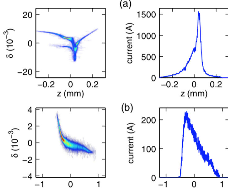
Figure 5. Samples of different longitudinal phase space (left column) and the corresponding current profiles (right column) for various settings in the dual linac and chicane shaping scheme. Adapted from [15].
