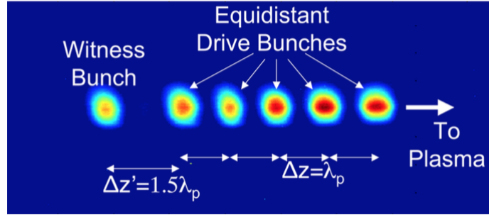
Figure 4. False-color image of bunch train used for PWFA experiments from masking method at BNL ATF. Adapted from Ref. [13].
