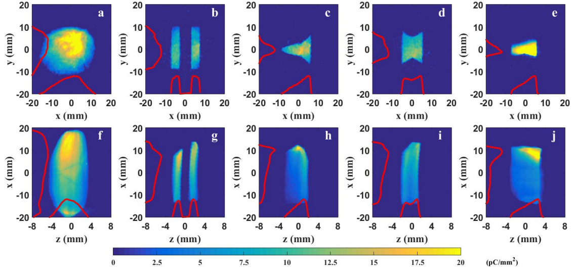
Figure 3. Longitudinal shaping by EEX beamline. The top row shows beam’s x - y image after the mask but before the exchange. The bottom row shows corresponding beam’s x - z image after the exchange. Figure is from Ref. [59]
