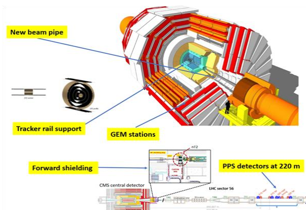
Fig. 1. Updated and new components of CMS for Run 3.
