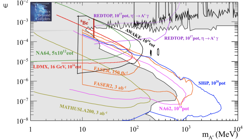
Fig. 15. Future upper limits at 90% CL for a minimal dark-photon model with visible decays in the plane mixing strength \epsilon versus mass m_{A'} for various projects on a \sim 10 –15 year timescale 74 .
