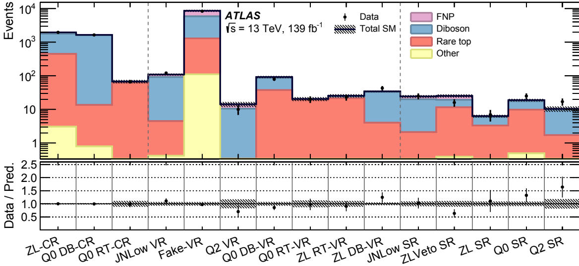
Figure 2: Observed and expected event yields in the CRs, VRs and SRs for the three- and four-lepton channels after the fit procedure described in the text. Diboson indicates background from diboson processes. Rare top indicates background from t\bar{t} + V and tWZ processes. FNP includes the background from fake or non-prompt leptons. Other indicates all the other considered backgrounds that contribute less than 2%. The hatched bands include systematic uncertainties with the correlations between various background sources taken into account. The lower panel shows the ratio of the observed data to the predicted SM background after the likelihood fit.
