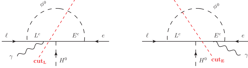
Figure 4: One-loop contributions to the g-2 of the SM leptons from the model Eq. (3.20), with the relevant 2-cuts.
