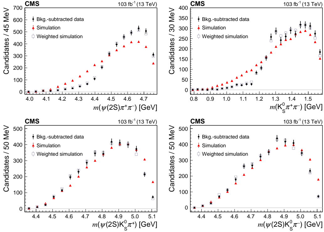
Figure 3: Distributions of 3-body intermediate invariant masses from the B^0 \rightarrow \psi(2S) K_S^0 \pi^+ \pi^- decay. Data distributions (black dots) are background subtracted. Overlaid are the predictions of phase space simulations (red triangles), as well as the predictions after applying the reweighting procedure described in Section 7 (grey squares).
