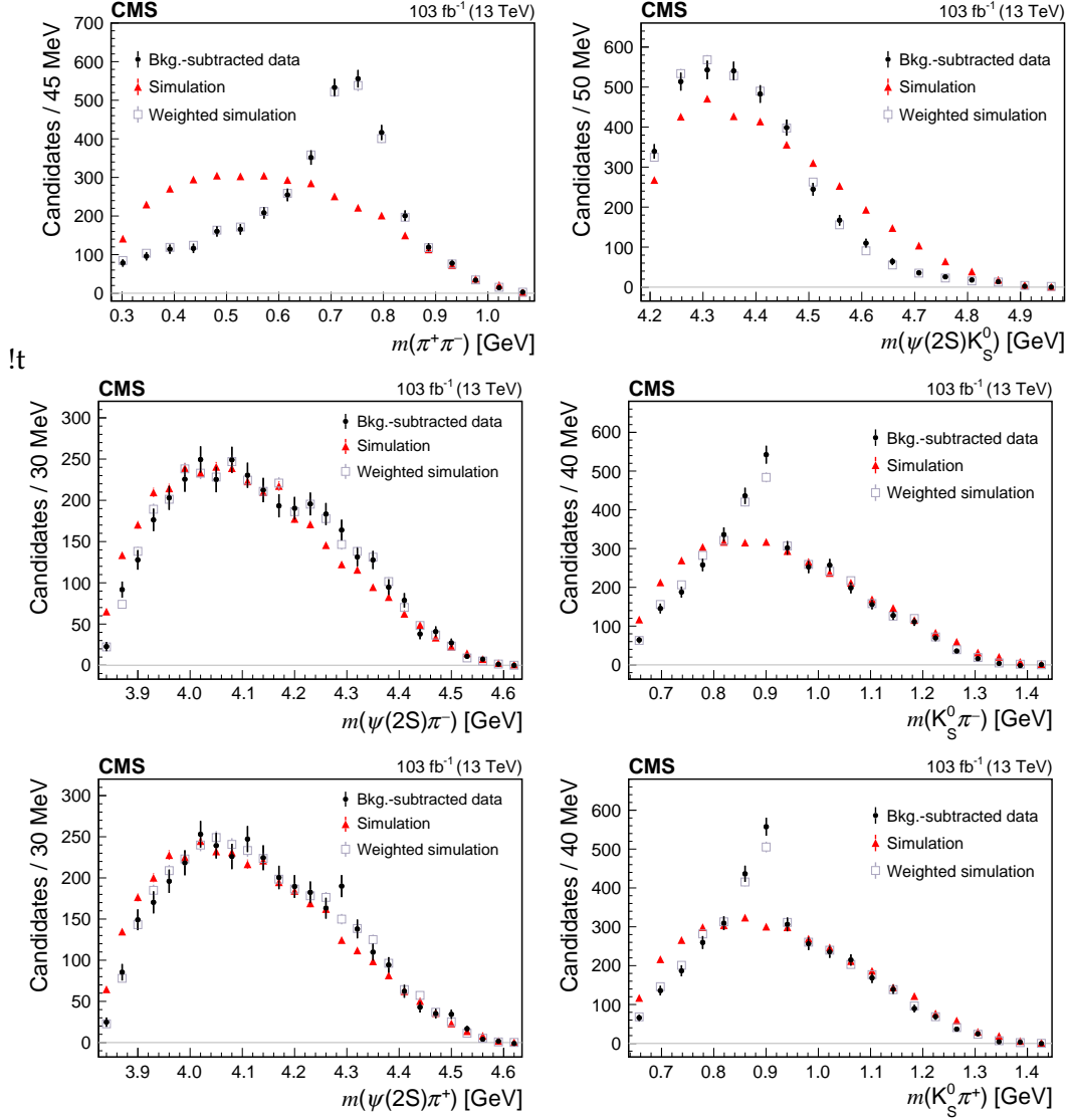
Figure 2: Distributions of 2-body intermediate invariant masses from the B^0 \rightarrow \psi(2S)K_S^0\pi^+\pi^- decay. The data distributions (black dots) are background subtracted. Overlaid are the predictions of phase space simulations (red triangles), as well as the predictions after applying the reweighting procedure described in Section 7 (grey squares).
