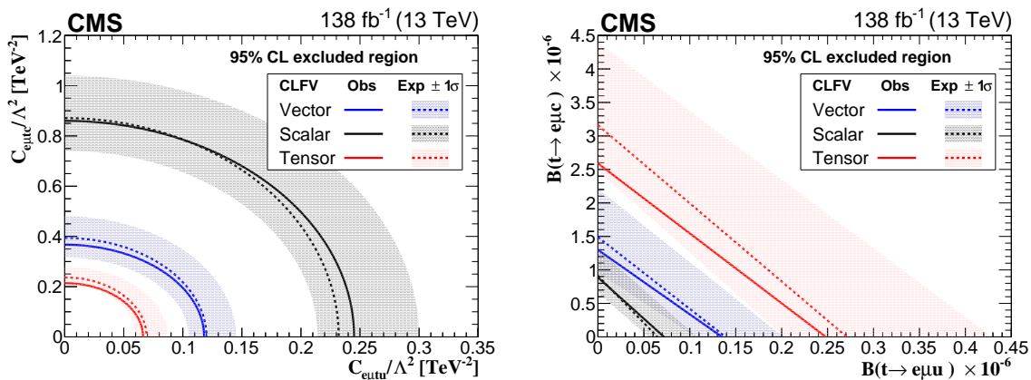
Figure 5: The observed 95% CL exclusion limits on the e\mu tc ; of the e\mu tu Wilson coefficient (left) and \mathcal{B}(t \rightarrow e\mu c) as a function of \mathcal{B}(t \rightarrow e\mu u) (right) for the vector-, scalar-, and tensor-like CLFV interactions. The hatched bands indicate the regions containing 68% of the distribution of limits expected under the background-only hypothesis.
