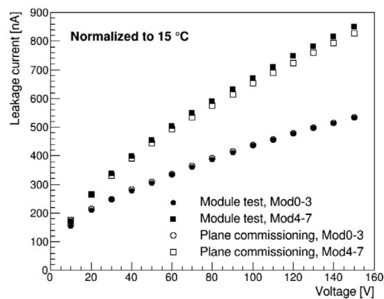
Fig. 27. Comparison of leakage current measurements during single module testing and plane commissioning.
