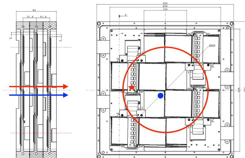
Fig. 12. Side (left) and front (right) views of a tracker station. The circle represents the 200mm-diameter magnet aperture, i.e. the acceptance of the tracker station. The blue dot and red star markers respectively correspond to the reference positions for material calculation in the central and edge regions.
