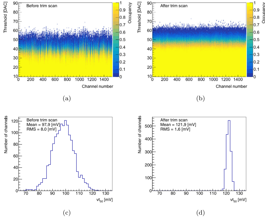
Fig. 29. Threshold scan for an example module with 1.5 fC injected charge before (a), and after (b) optimal trim settings from the trim scan are applied. The distributions of the v_{50} points for all strips are also shown before (c), and after (d) the trim scan.
