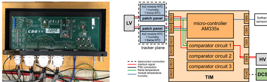
Fig. 20. TIM board and corresponding block diagram (signal path shown for only two patch-panels, while six patch-panels can be fed).
