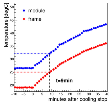
Fig. 22. Thermal behavior of frame and module in case of a cooling stop. A special single plane was used for this test and all protection mechanisms were deactivated. The dashed lines indicates the moment when the hardware interlock would become active. The actual module temperature is still well below 35.0^\circ\text{C} .
