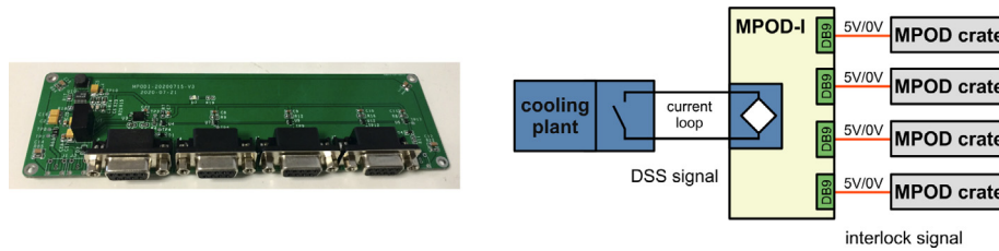
Fig. 21. MPOD-I board and corresponding block diagram.
