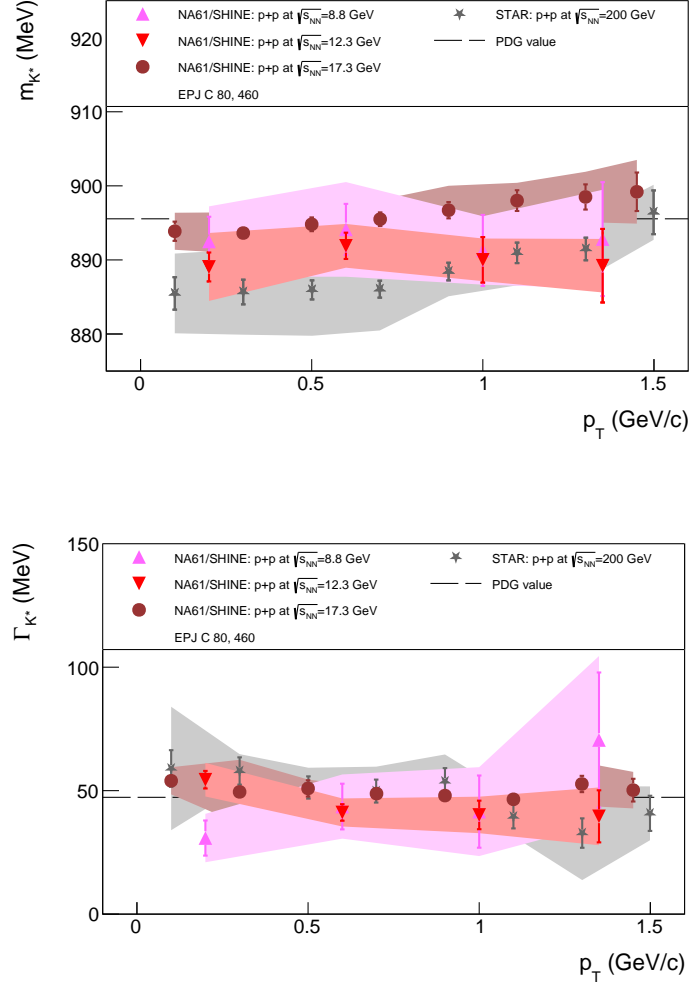
Figure 10.: The transverse momentum dependence of mass and width of K^*(892)^0 (or K^{*0} ) mesons obtained in p+p collisions by NA61/SHINE (this analysis and Ref. [9]) and STAR [11]. For STAR the averaged ( K^{*0} ) measurements of K^*(892)^0 and \bar{K}^*(892)^0 are presented. The horizontal lines represent PDG values [28].
