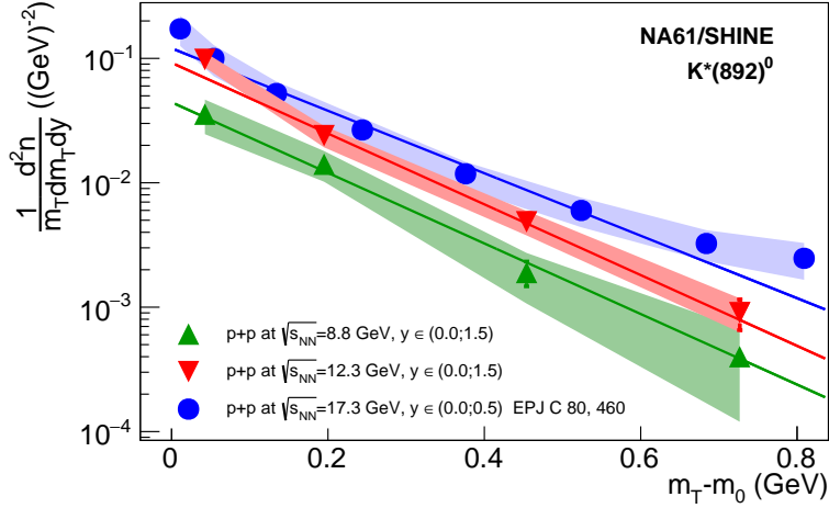
Figure 7.: The transverse mass spectra \frac{1}{m_T} \frac{d^2n}{dm_T dy} of K^*(892)^0 mesons produced in inelastic p+p collisions at 40 GeV/c and 80 GeV/c in rapidity range 0 < y < 1.5 . The numerical values are listed in Table 6. The solid lines represent function given by Eqs. (11) and (12) with A and T parameters taken from Fig. 6. For a comparison the previous NA61/SHINE results [9] for p+p interactions at 158 GeV/c are also shown (they were obtained in 0 < y < 0.5 ).
