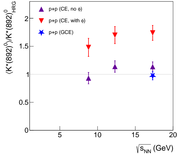
Figure 12.: The \langle K^*(892)^0 \rangle NA61/SHINE values measured in inelastic p+p collisions at p_{\text{beam}} = 40\text{--}158 GeV/c (this analysis and Ref. [9]), divided by the Hadron Resonance Gas model predictions within the Canonical Ensemble [37] for the fit with \phi mesons included (upside-down triangles) and the fit with \phi meson excluded (triangles). The star shows the \langle K^*(892)^0 \rangle [9] divided by the HRG model prediction for the Grand Canonical Ensemble [37, 38]. The numerical values of \langle K^*(892)^0 \rangle and K^*(892)^0_{\text{HRG}} are listed in Table 9 of Appendix A.
