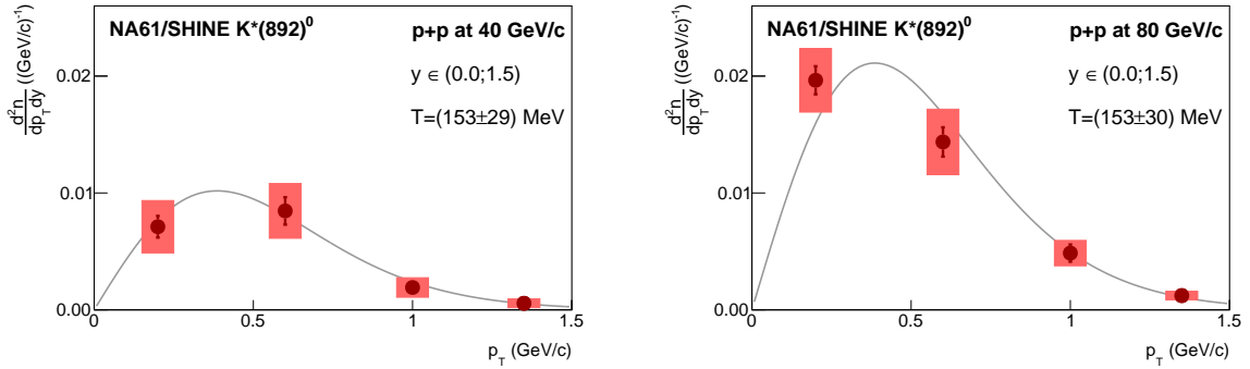
Figure 6.: The transverse momentum spectra \frac{d^2n}{dy dp_T} of K^*(892)^0 mesons produced in inelastic p+p collisions at 40 GeV/c (left) and 80 GeV/c (right) in rapidity range 0 < y < 1.5 . The fitted function (solid line) is given by Eq. (11). The numerical values are listed in Table 5. The fitted inverse slope parameters T are quoted in the legends.
