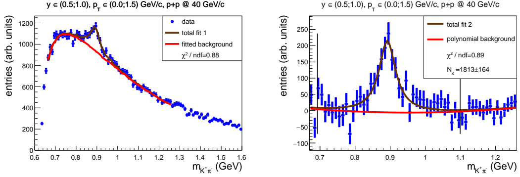
Figure 3.: The example of the procedure of signal extraction for K^*(892)^0 in rapidity bin 0.5 < y < 1.0 (all rapidity values in the paper are given in the center-of-mass reference system) and transverse momentum range 0 < p_T < 1.5 GeV/c for p+p collisions at 40 GeV/c. Left: data signal (blue points) and fitted background (red line) obtained from the templates. Right: background-subtracted signal – more details in the text. Thin black vertical lines in the right panel correspond to the range of integration of the fit functions when obtaining the raw number of K^*(892)^0 mesons ( m_0 \pm 4\Gamma_0 ).
