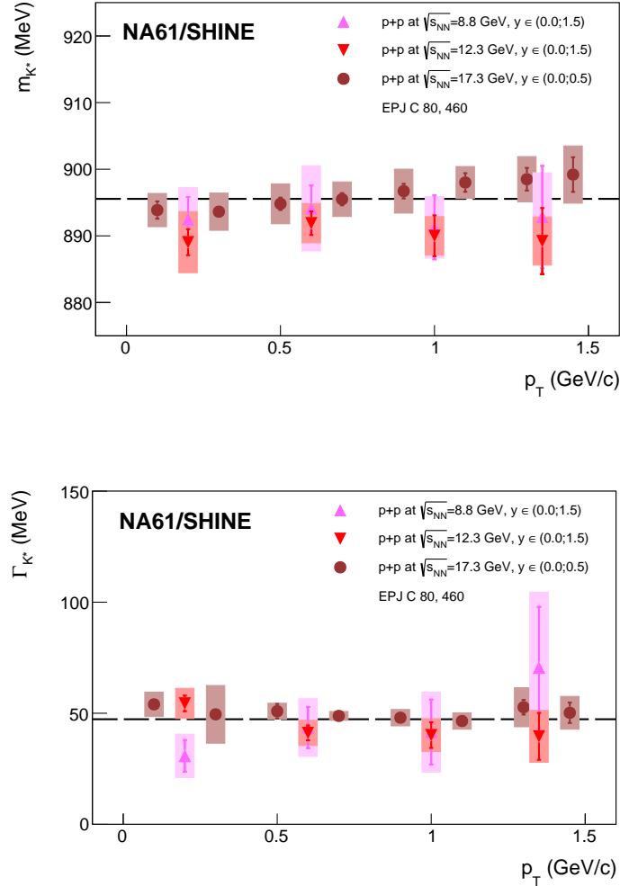
Figure 5.: The transverse momentum dependence of mass (top) and width (bottom) of K^*(892)^0 mesons obtained in inelastic p+p collisions at 40 GeV/c and 80 GeV/c ( \sqrt{s_{NN}} = 8.8 and 12.3 GeV) in rapidity range 0 < y < 1.5 . The numerical data are listed in Table 4. The dashed horizontal lines represent PDG values m_0 = 895.55 MeV and \Gamma_0 = 47.3 MeV [28]. For a comparison the previous NA61/SHINE results [9] for p+p interactions at 158 GeV/c ( \sqrt{s_{NN}} = 17.3 GeV) are also shown (they were obtained in 0 < y < 0.5 ).
