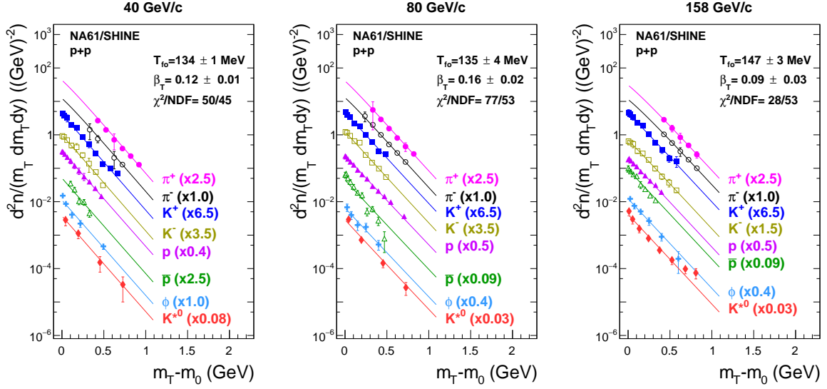
Figure 14.: The transverse mass spectra of K^*(892)^0 mesons ( 0 < y < 1.5 for 40 and 80 GeV/c from this analysis, and 0 < y < 0.5 for 158 GeV/c from Ref. [9]) and other hadrons previously measured by NA61/SHINE (charged pions, charged kaons, protons, anti-protons [40] in 0 < y < 0.2 , and \phi mesons [41] in 0 < y < 0.3 ; for \pi^- at 80 GeV/c the rapidity range 0.2 < y < 0.4 was used instead of 0 < y < 0.2 ) fitted within the BW model [6] described by Eq. (18). Results for 40 GeV/c (left), 80 GeV/c (middle), and 158 GeV/c (right) beam momenta. For all points the vertical uncertainty bars represent total uncertainties (square root of the sum of squares of statistical and systematic uncertainties). The fits were performed in the range 0 < m_T - m_0 < 1 GeV. The resulting fit parameters are displayed in the legends.
