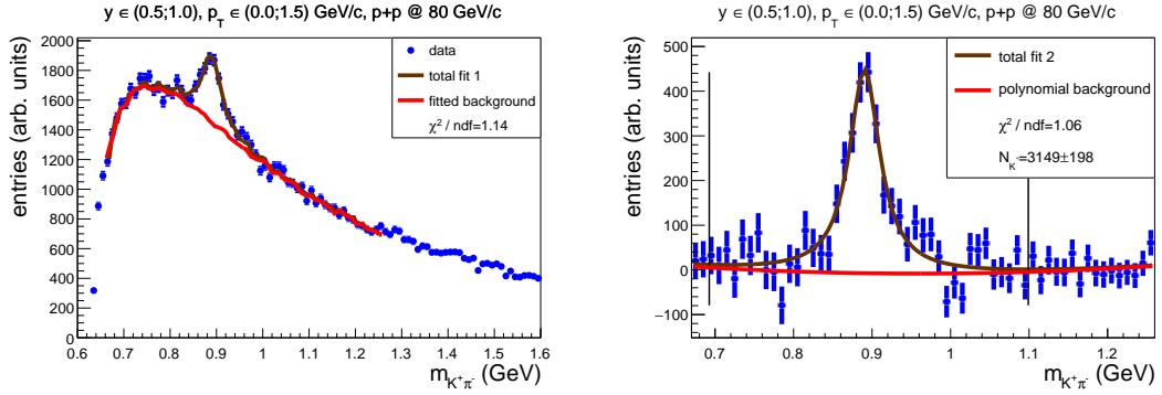
Figure 4.: Same as Fig. 3 but for p+p collisions at 80 GeV/c.
