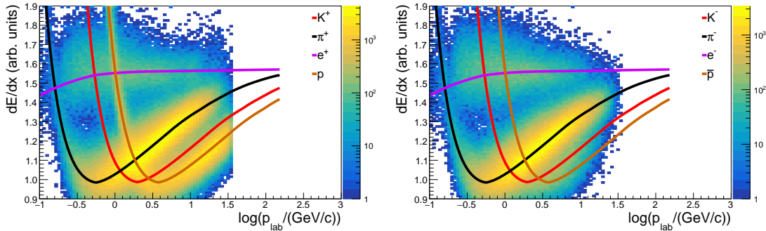
Figure 2.: The values of dE/dx versus \log(p_{lab}/(\text{GeV}/c)) for positively (left) and negatively (right) charged particles after track cuts (i) – (vi) from Sec. 3.4. Data for inelastic p+p collisions at 40 GeV/c beam momentum. The empirical parametrizations of Bethe-Bloch curves are also drawn.
