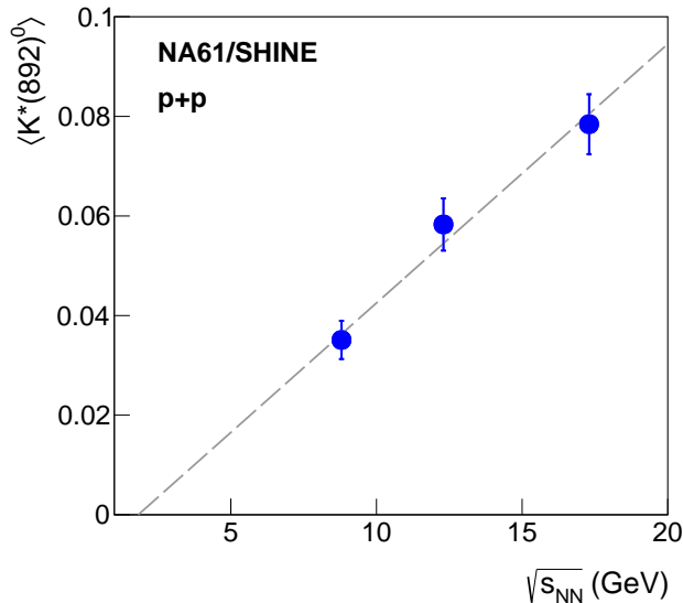
Figure 9.: The energy dependence of \langle K^*(892)^0 \rangle in inelastic p+p collisions. The previous NA61/SHINE result [9] for p+p interactions at 158 GeV/c is also shown. The mean multiplicities were obtained for 0 < p_T < 1.5 GeV/c (two lower energies, this analysis) or for the full phase space [9] (the highest energy). The vertical bars represent the total uncertainties (square root of the sum of squares of statistical and systematic uncertainties). The dashed line is added as a guide to the eye.
