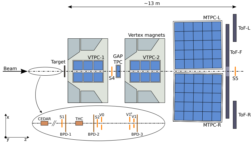
Figure 1.: The schematic layout of the NA61/SHINE spectrometer (horizontal cut, not to scale) used for p+p data taking. The beam and trigger detector configuration is shown in the inset (see Refs. [23,24] for detailed description). The chosen coordinate system is drawn on the lower left: its origin lies in the middle of the VTPC-2, on the beam axis.
