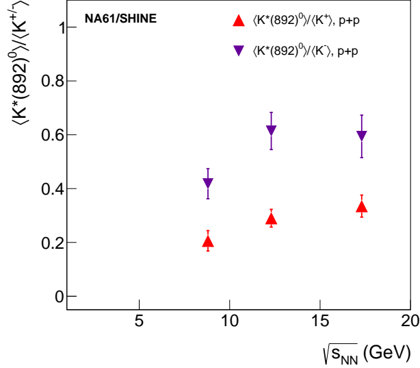
Figure 13.: The \langle K^*(892)^0 \rangle / \langle K^+ \rangle and \langle K^*(892)^0 \rangle / \langle K^- \rangle yield ratios obtained in inelastic p+p collisions at p_{beam} = 40 – 158 GeV/c. The numerical values are given in Table 10 of Appendix A ( p+p at 40 and 80 GeV/c) and in Ref. [9] (NA61/SHINE p+p data at 158 GeV/c).
