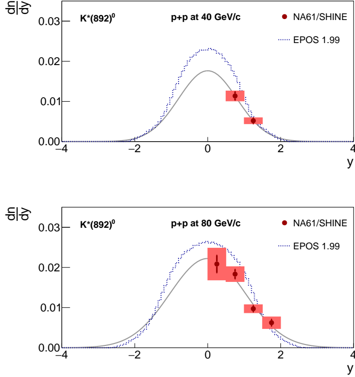
Figure 11.: The comparison of K^*(892)^0 rapidity distributions from NA61/SHINE (points) and the Epos1.99 model (dotted lines). Results for inelastic p+p collisions at 40 GeV/c (top) and 80 GeV/c (bottom). The fitted Gaussian functions to NA61/SHINE points (gray solid lines) are given by Eq. (13).
