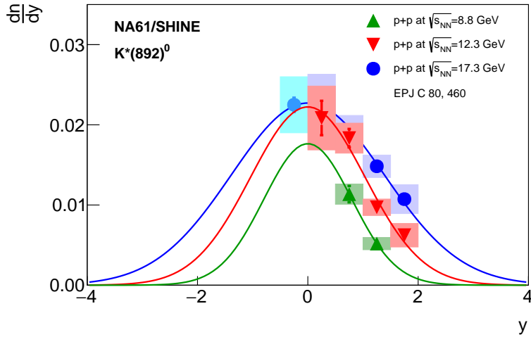
Figure 8.: The rapidity spectra \frac{dn}{dy} of K^*(892)^0 mesons produced in inelastic p+p collisions at 40 GeV/c and 80 GeV/c in transverse momentum range 0 < p_T < 1.5 GeV/c. The numerical values are listed in Table 7. The solid lines represent the function given by Eq. (13). For comparison the previous NA61/SHINE results [9] for p+p interactions at 158 GeV/c are also shown (they were obtained in the full transverse momentum range; p_T -integrated and extrapolated rapidity spectrum). For 158 GeV/c the first (light blue) point ( y < 0 ) was not included in the fit (see Ref. [9] for details).
