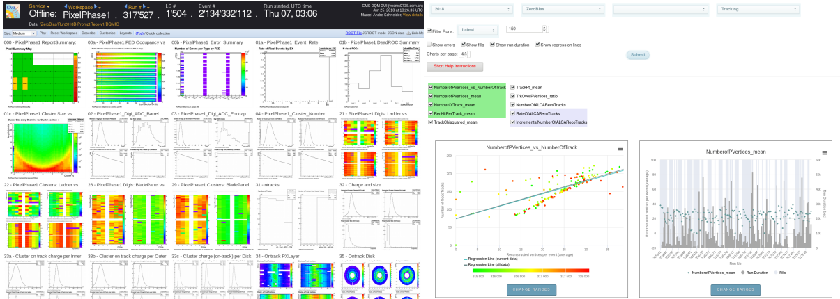
Figure 2. The user interface of DQMGUI (left) and historic DQM (right).
