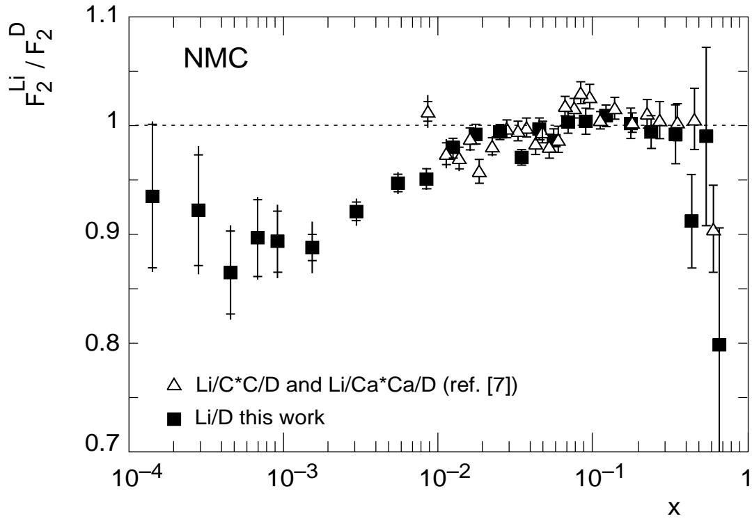
Figure 8: The present result for F_2^{\text{Li}/\text{D}} compared to the indirect result obtained by multiplying F_2^{\text{Li}}/F_2^{\text{C}} and F_2^{\text{Li}}/F_2^{\text{Ca}} (90 GeV) with F_2^{\text{C}}/F_2^{\text{D}} and F_2^{\text{Ca}}/F_2^{\text{D}} (200 GeV), respectively [7]. The inner error bars represent the statistical errors, the outer ones the statistical and systematic errors added in quadrature. The relative normalisation uncertainty between the two results, not included in the figure, is 0.8%.
