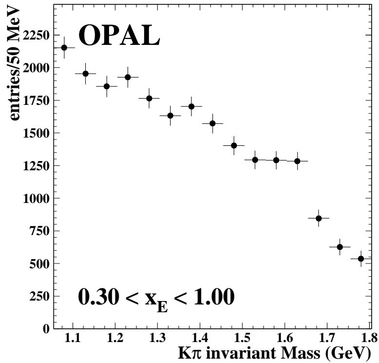
Figure 12: Invariant mass spectra for K\pi combinations around the K_2^*(1430)^0 mass.
