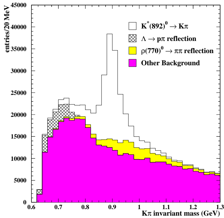
Figure 5: Composition of the 'subtracted' JETSET Monte Carlo K\pi mass spectrum.
