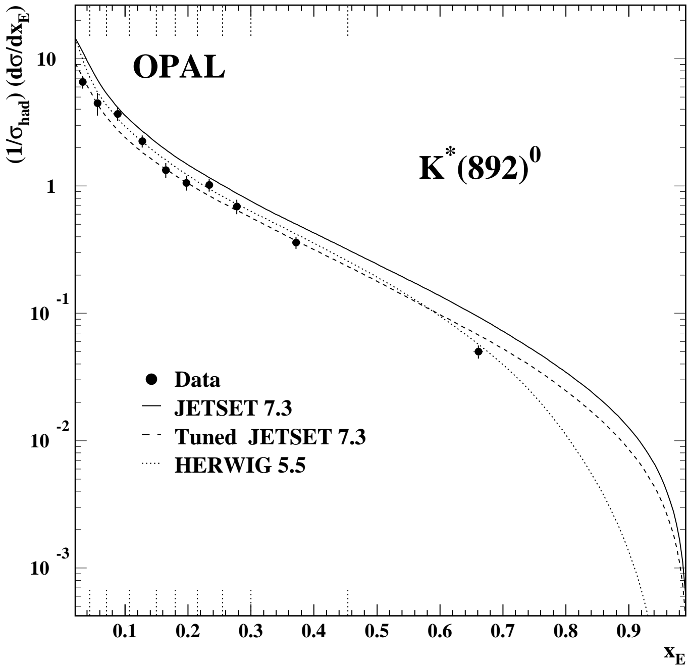
Figure 9: Differential cross sections for measured and simulated K^*(892)^0 production. The solid curve indicates the prediction of JETSET 7.3 using default parameters and the dashed curve shows the result of tuning JETSET as described in section 6.3. The HERWIG 5.5 prediction is displayed as a dotted curve. The error bars show the combined statistical and systematic uncertainty on each point. The bin ranges are indicated by means of the short vertical lines at the top and bottom of the plot.
