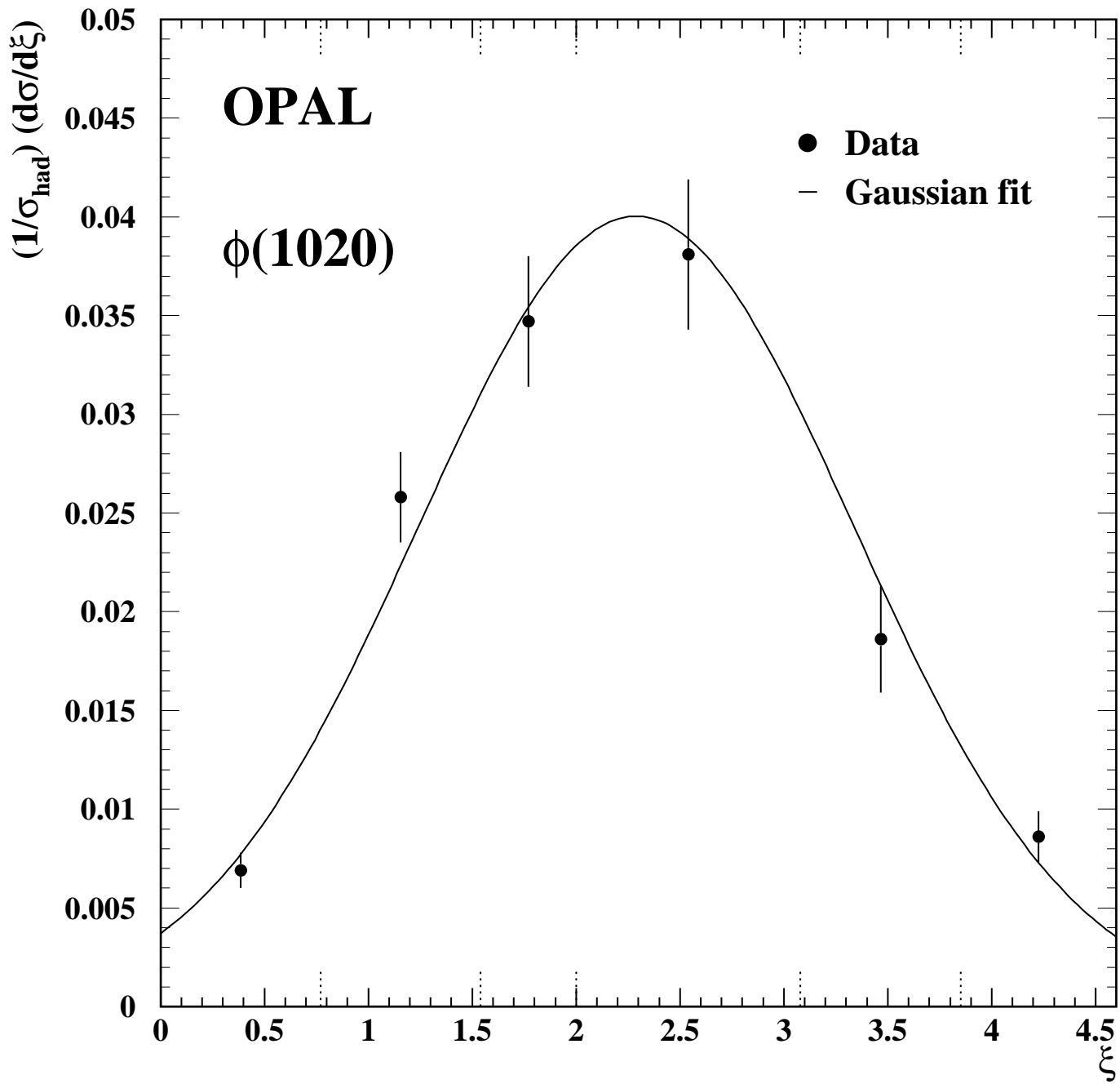
Figure 10: Differential cross section for \phi(1020) as a function of \xi = \ln(1/x_p) . The error bars show the combined statistical and systematic uncertainty on each point. The bin ranges are indicated by means of the short vertical lines at the top and bottom of the plot.
