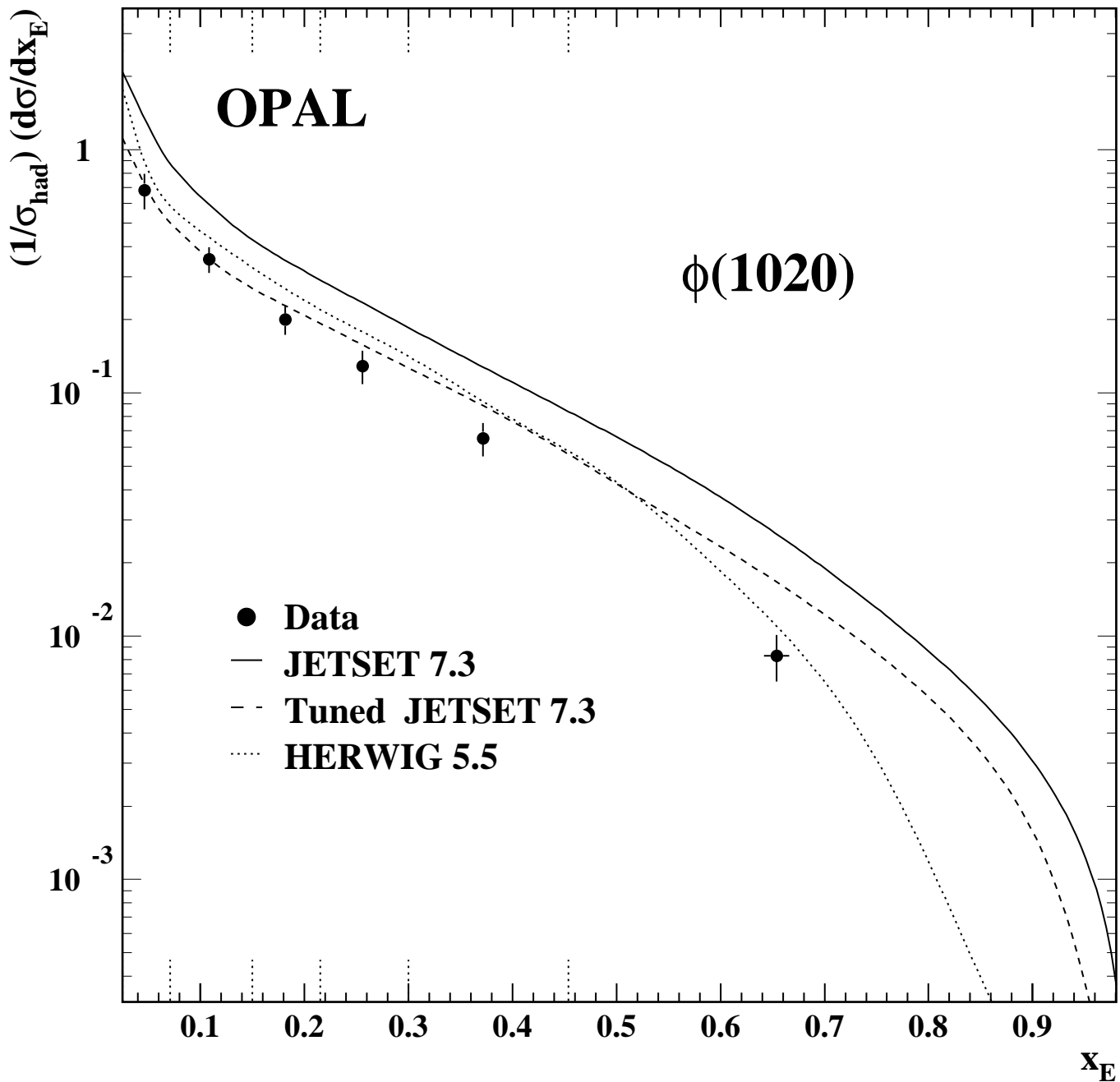
Figure 8: Differential cross sections for measured and simulated \phi(1020) production. The solid curve indicates the prediction of JETSET 7.3 using default parameters and the dashed curve shows the result of tuning JETSET as described in section 6.3. The HERWIG 5.5 prediction is displayed as a dotted curve. The error bars show the combined statistical and systematic uncertainty on each point. The bin ranges are indicated by means of the short vertical lines at the top and bottom of the plot.
