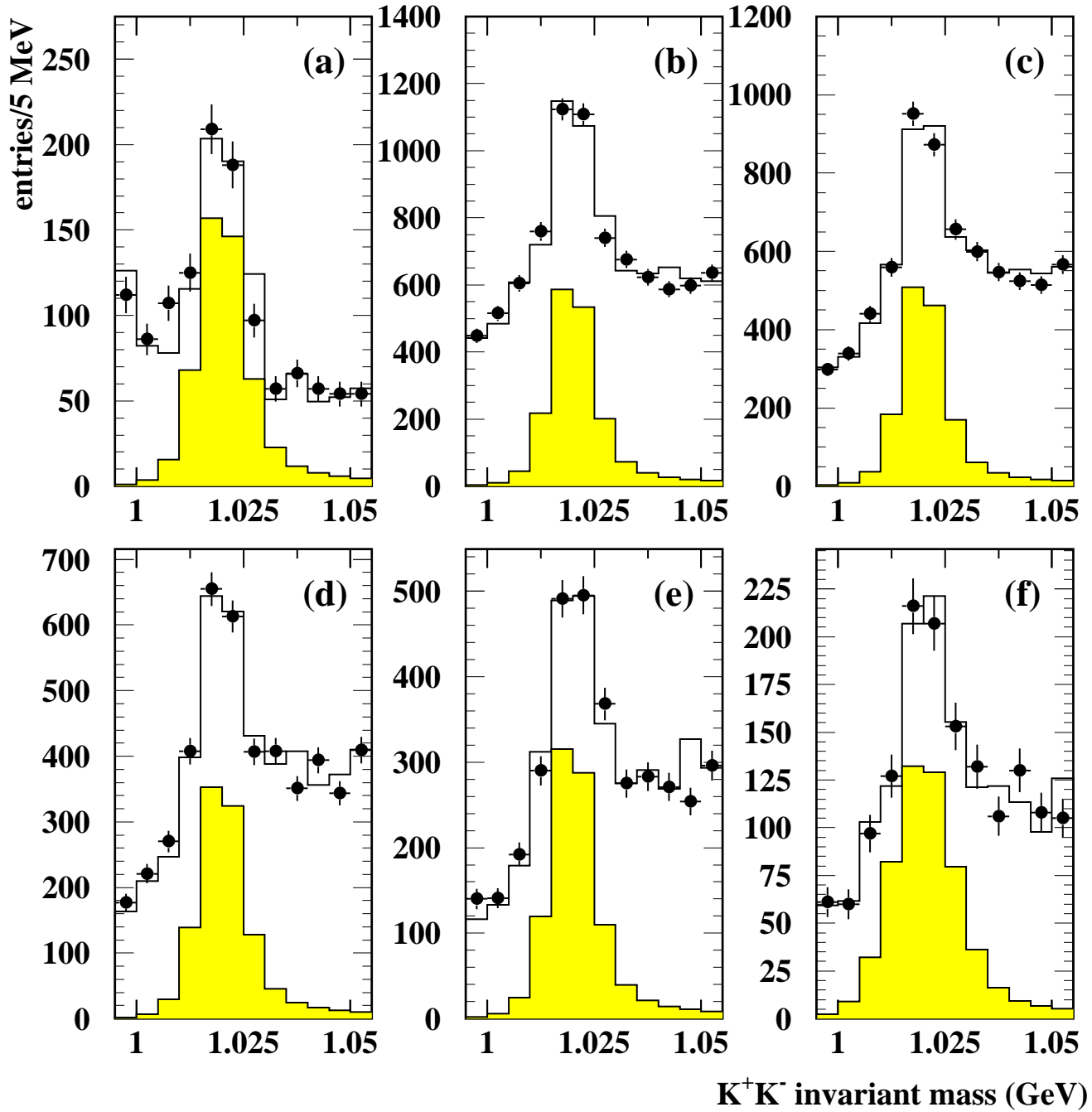
Figure 6: Fits to the K^+K^- invariant mass plots in six bins of x_E : (a) 0.025 < x_E < 0.071 , (b) 0.071 < x_E < 0.150 , (c) 0.150 < x_E < 0.215 , (d) 0.215 < x_E < 0.300 , (e) 0.300 < x_E < 0.454 , (f) 0.454 < x_E < 1.000 . The open histograms show the results of the fits, and the shaded plots are the extracted \phi(1020) signals.
