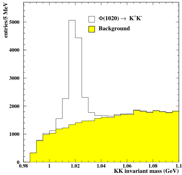
Figure 4: Composition of the JETSET Monte Carlo K^+K^- mass spectrum.
