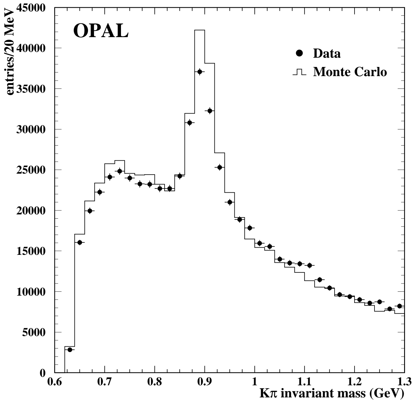
Figure 3: Two-particle ‘subtracted’ invariant mass spectra for selected K\pi combinations.
