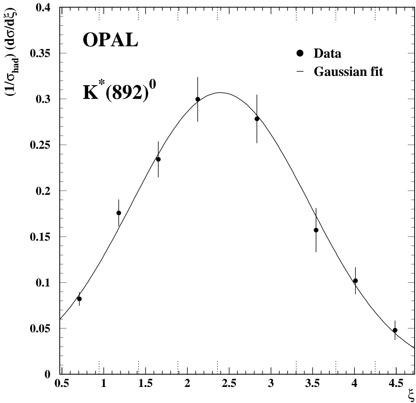
Figure 11: Differential cross section for K^*(892)^0 as a function of \xi = \ln(1/x_p) . The error bars show the combined statistical and systematic uncertainty on each point. The bin ranges are indicated by means of the short vertical lines at the top and bottom of the plot.
