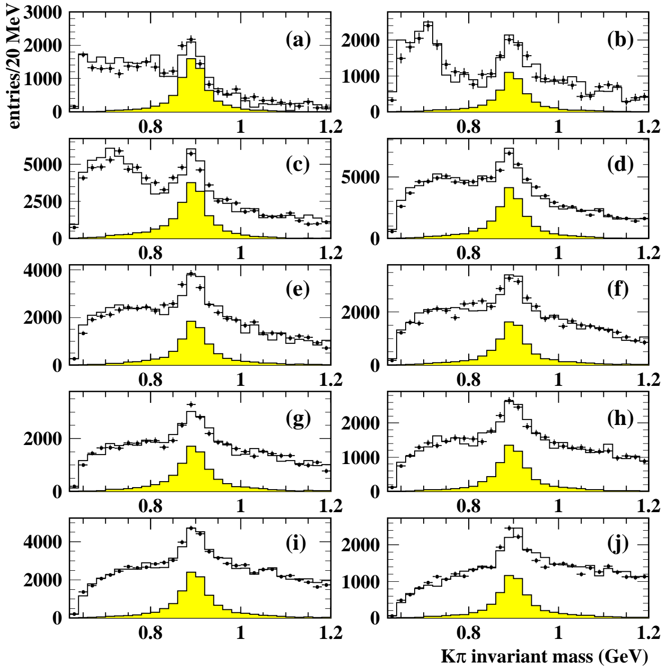
Figure 7: Fits to the K\pi invariant mass plots in ten bins of x_E : (a) 0.021 < x_E < 0.044 , (b) 0.044 < x_E < 0.071 , (c) 0.071 < x_E < 0.107 , (d) 0.107 < x_E < 0.150 , (e) 0.150 < x_E < 0.180 , (f) 0.180 < x_E < 0.215 , (g) 0.215 < x_E < 0.255 , (h) 0.255 < x_E < 0.300 , (i) 0.300 < x_E < 0.454 , (j) 0.454 < x_E < 1.000 . The open histograms show the results of the fits, and the shaded plots are the extracted K^*(892)^0 signals.
