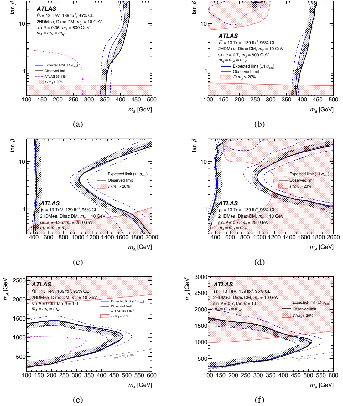
Figure 5: Exclusion limits within the context of 2HDM+a models with different parameter choices and in various planes [17]. Subfigures (a, b) show the \tan \beta vs m_a exclusion limits with m_A = 600 \text{ GeV} , (c, d) the \tan \beta vs m_A exclusion limits with m_a = 250 \text{ GeV} , and (e, f) the m_A vs m_a exclusion limit with \tan \beta = 1.0 . The region contained by the solid black line and the hashed black contour is excluded at the 95% CL. The solid blue line indicates the expected limit in the absence of signal, and the dashed blue lines the corresponding \pm 1 \sigma uncertainty band. Subfigures (a, c, e) assume \sin \theta = 0.35 , while (b, d, f) assume \sin \theta = 0.7 . Where included, the dashed magenta lines represent the 36.1 \text{ fb}^{-1} results from Ref. [18]. The hashed red area indicates that the width of one of the Higgs bosons is larger than 20% of its mass.
