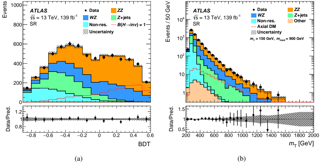
Figure 3: (a) BDT and (b) m_T distributions in the signal region, after the respective simultaneous fits. The H \rightarrow \text{inv} signal, with a branching ratio of \mathcal{B} = 100\% , is shown in (a) and an example DM axial-vector signal with (m_\chi, m_{\text{med}}) = (150, 900) GeV is shown in (b). As defined in the text, ‘Non-res.’ includes WW , t\bar{t} , single top-quark and Z \rightarrow \tau\tau processes, while ‘Other’ stands for triboson, t\bar{t} + V , and ZZ \rightarrow 4\ell production. Events recorded below (above) the x -range of the BDT plot are included in the first (last) bin shown. The bottom panel in each figure shows the ratio of the observed data to the predicted yields. The shaded bands in top and bottom panels represent the total statistical and systematic error of the background.
