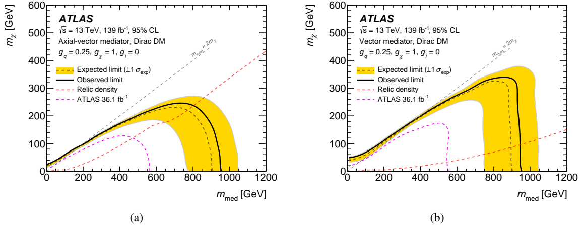
Figure 4: Exclusion limits for simplified DM models with g_\chi = 1.0 , g_q = 0.25 , and g_\ell = 0 , when assuming (a) an axial-vector mediator or (b) a vector mediator. The region below the solid black line is excluded at the 95% CL. The dashed black line indicates the expected limit in the absence of signal, and the yellow band the corresponding \pm 1\sigma uncertainty band. The dashed red line labelled ‘Relic density’ corresponds to combinations of DM and mediator mass values that are consistent with a DM density of \Omega h^2 = 0.118 and a standard thermal history, as computed in Ref. [13]. Below the line, annihilation processes described by the simplified model mostly predict too high a relic density while regions with too low a relic density are mostly found for m_{\text{med}} closer to the DM mass. The dashed magenta line indicates the previous ATLAS result from a 36.1 \text{ fb}^{-1} dataset [23].
