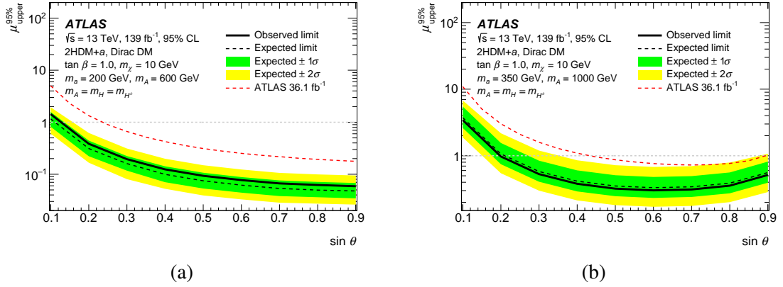
Figure 6: \sin \theta exclusion limits for 2HDM+a signals with \tan \beta = 1.0 and m_\chi = 10 GeV. The solid black line shows the observed limit, while the dashed black line indicates the expected limit in the absence of signal, with the corresponding 1\sigma and 2\sigma uncertainty bands in green and yellow. The dashed red line shows the result from the 36 \text{ fb}^{-1} analysis [18]. The region below \mu_{\text{upper}}^{95\%} = 1 is excluded at the 95% CL. In (a), m_A = 600 GeV and m_a = 200 GeV, while in (b) m_A = 1000 GeV and m_a = 350 GeV.
