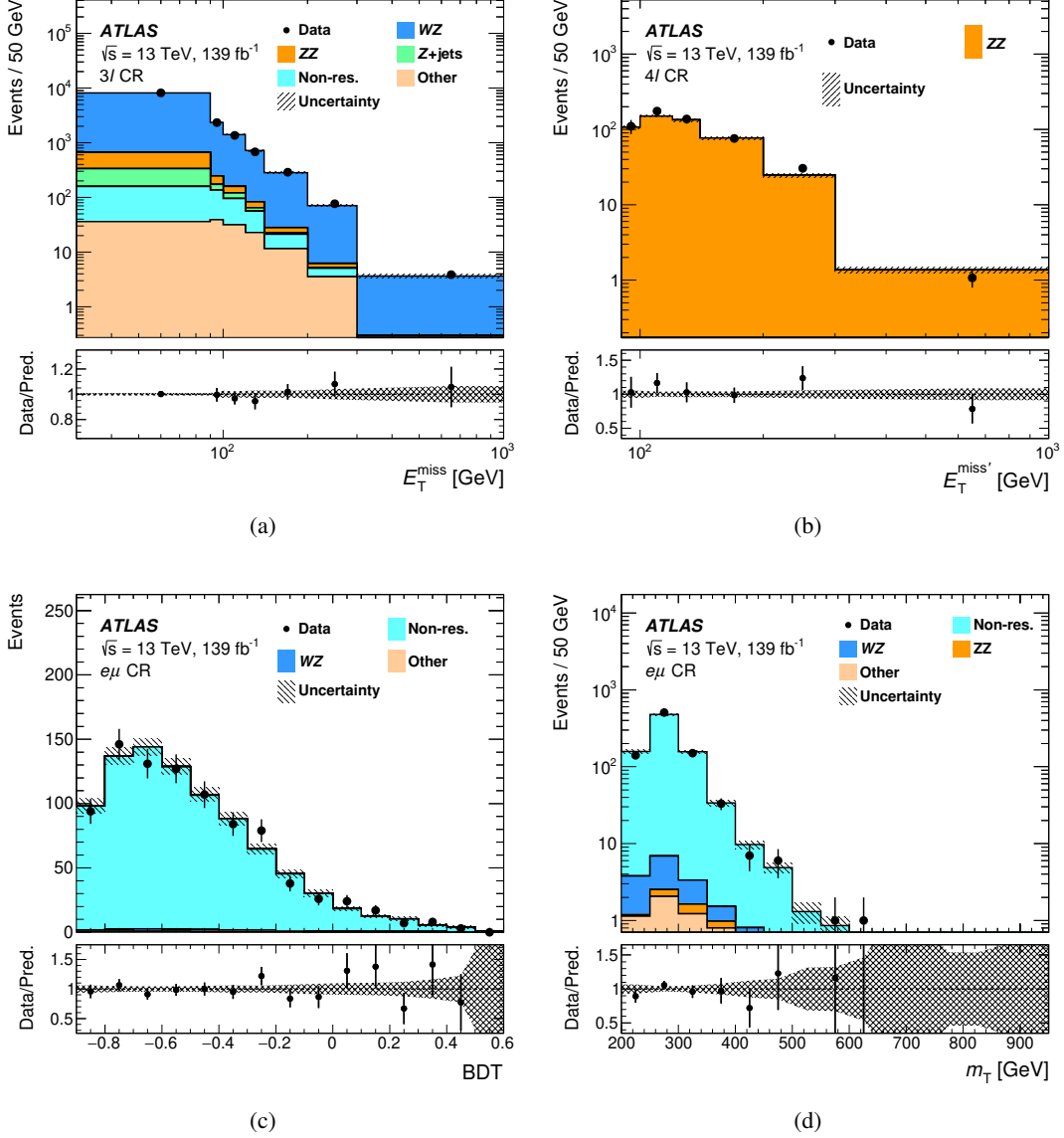
Figure 2: Distributions in data compared with simulated events in the different CRs after (a, b, c) the simultaneous ZH \rightarrow \ell\ell + \text{inv} fit and (d) a fit in the context of the simplified DM models (axial-vector signal with (m_\chi, m_{\text{med}}) = (150, 900) GeV): (a) E_T^{\text{miss}} distribution in the 3 \ell CR, (b) E_T^{\text{miss}'} distribution in the 4 \ell CR, (c) BDT distribution in the e\mu CR, (d) m_T distribution in the e\mu CR. As defined in the text, ‘Non-res.’ includes WW , t\bar{t} , single-top and Z \rightarrow \tau\tau processes, while ‘Other’ stands for triboson, t\bar{t} + V , and ZZ \rightarrow 4\ell production. Events recorded below (above) the x -range of the BDT plot are included in the first (last) bin shown. The bottom panel in each figure shows the ratio of the observed data to the predicted yields. The shaded bands in top and bottom panels represent the total statistical and systematic error of the background.
