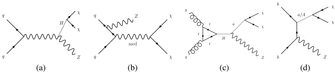
Figure 1: Example Feynman diagrams of the probed processes: (a) associated production of a Higgs boson and a Z boson, where the Higgs boson decays into DM particles, (b) production of a Z boson and a mediator from a quark initial state in the simplified DM models, and (c) gg - and (d) bb -initiated 2HDM+ a diagrams.
