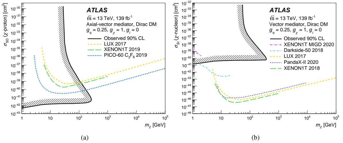
Figure 8: Comparison of the upper limits at 90% CL from direct-detection experiments [1–8] with the exclusion obtained in the simplified DM models in the plane of the dark matter mass and (a) the spin-dependent WIMP–proton scattering cross-section or (b) the spin-independent WIMP–nucleon scattering cross-section [12]. The area within the shaded lines is excluded by this analysis in the context of the simplified models.
