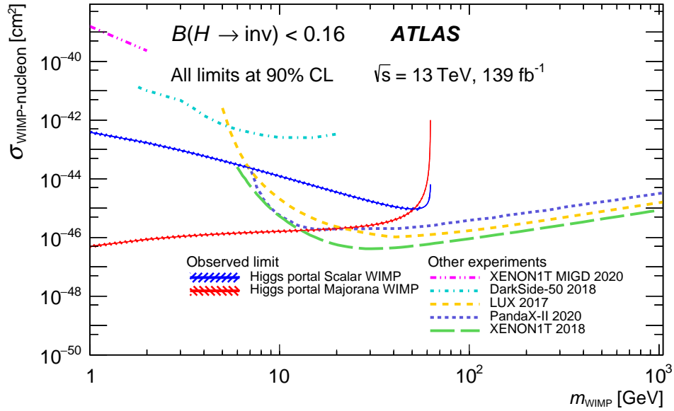
Figure 7: Comparison between the 90% CL upper limits on the spin-independent WIMP–nucleon scattering cross-section from direct-detection experiments [1–5] and a reinterpretation of the \mathcal{B}(H \rightarrow \text{inv}) limit obtained in this analysis, as a function of the WIMP mass. Higgs portal scenarios are assumed, where the 125 GeV Higgs boson decays into a pair of DM particles [104] that are either scalars or Majorana fermions. The uncertainties from the nuclear form factor are indicated by the hatched band. The regions above the limit contours are excluded in the \sigma_{\text{WIMP-N}} range shown in the plot.
