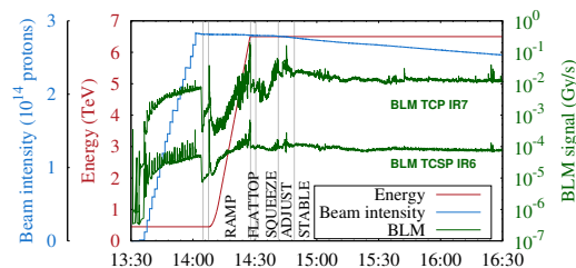
Figure 1: Time profile of BLM signals in IR6 and IR7 during a representative proton fill (19/10/2018). The different operational phases are indicated by the vertical grey lines. For both insertion regions, a BLM located near a collimator was chosen.
