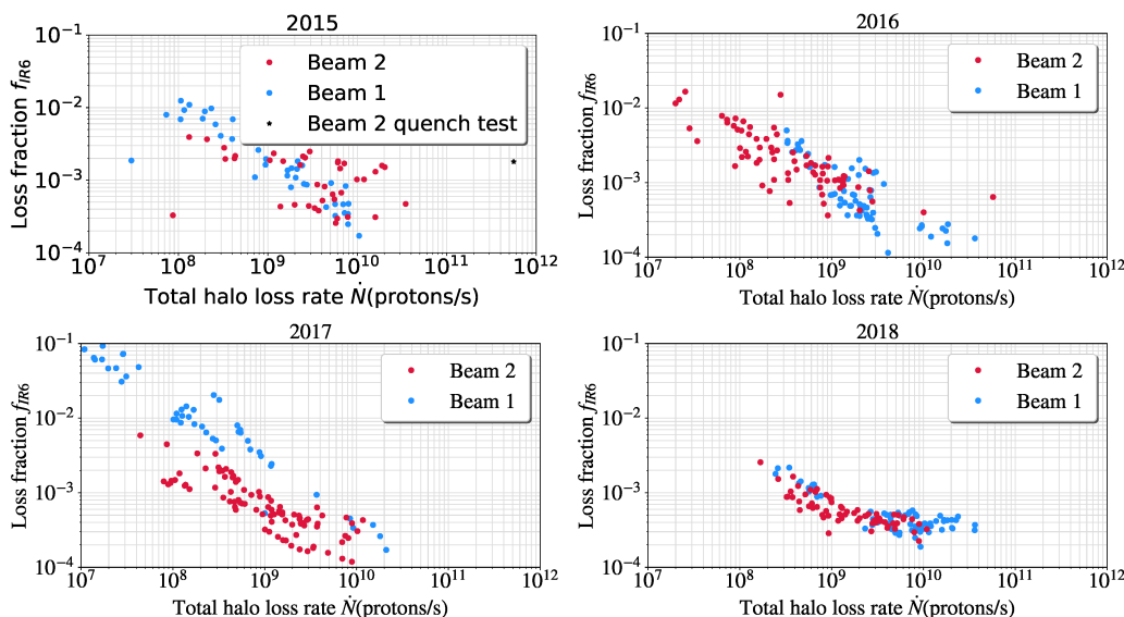
Figure 2: Analysis of proton leakage from IR7 to IR6 during high loss events in Run 2.
