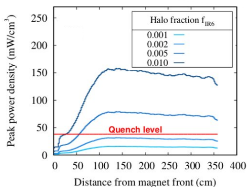
Figure 3: Peak power density in the coils of the Q4 magnet (IR6) for a 0.2 h beam lifetime in HL-LHC. Results were normalized to different halo fractions f_{IR6} .
