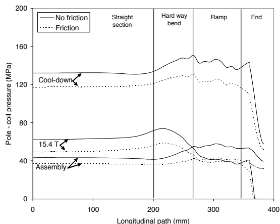
Fig. 7. Contact pressure between winding pole and coil layer 1: results are given along the longitudinal path, located at the middle of the layer, and moving from the straight section center ( z = 0 mm) to the end ( z = 384 mm).
