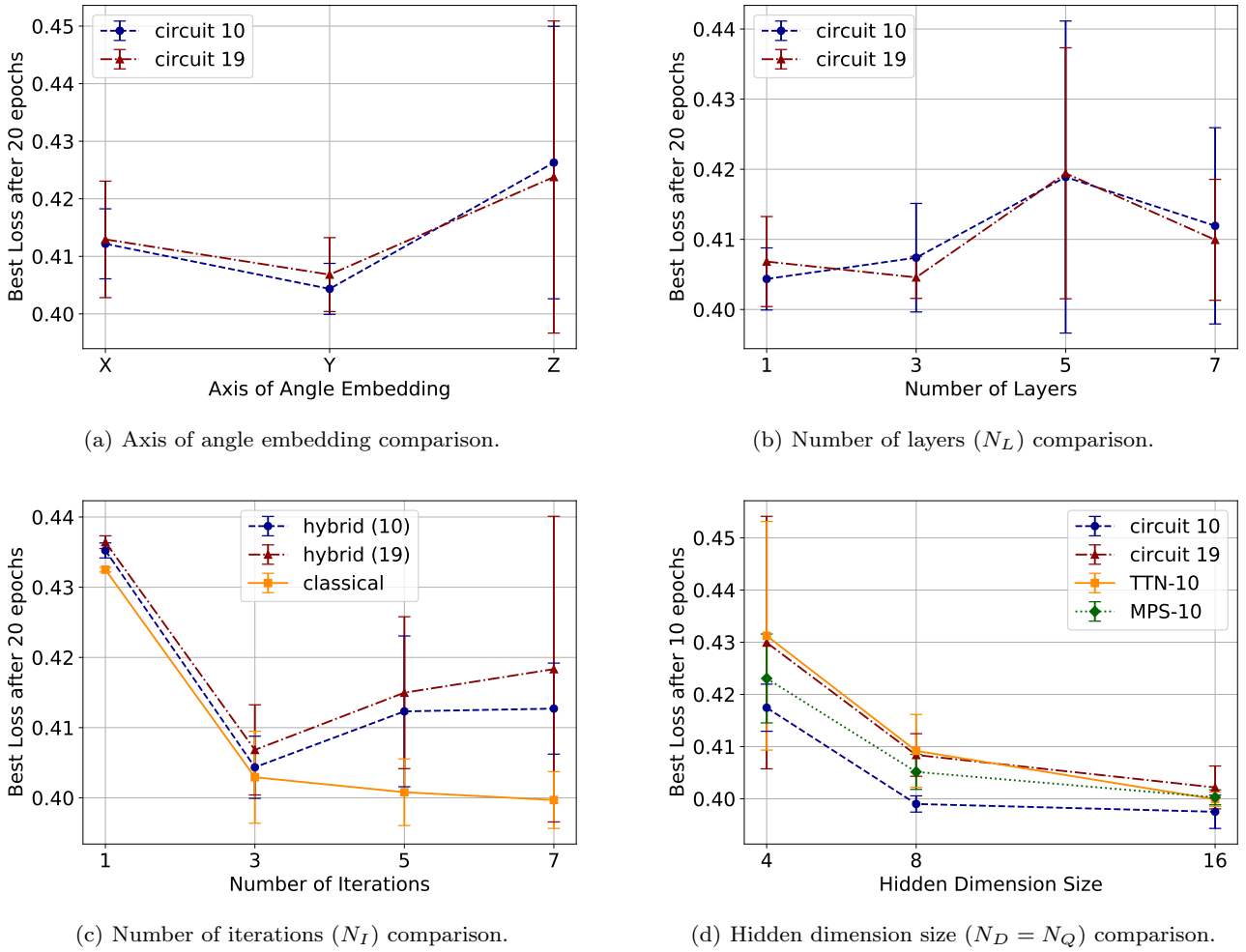
Fig. 9 Best validation loss comparison with respect to different parameters of the hybrid GNN model. (a) The axis of angle embedding comparison considers the best loss obtained for different embedding axes by setting N_D = N_Q = 4 , N_L = 1 and N_I = 3 . (b) The number of layers comparison considers the best loss for various numbers of layers ( N_L ) by setting N_D = N_Q = 4 and N_I = 3 . (c) The number of iterations comparison considers the best loss for different numbers of iterations ( N_I ) by setting N_D = N_Q = 4 and N_L = 1 . (d) The hidden dimension size comparison considers the loss for different hidden dimension sizes ( N_D ) by setting N_Q = N_D , N_L = 1 and N_I = 3 . 5 instances of all models with different initial parameters are trained for 10 or 20 epochs depending on complexity for each setting, and the mean of best losses are presented. The error bars represent the \pm standard deviation of the best losses of all 5 runs.
