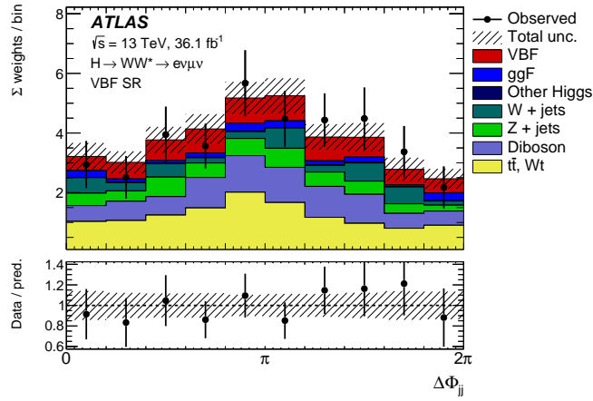
Figure 7: The weighted \Delta\Phi_{jj} distribution in the VBF signal region, with signal and background yields fixed from the fit for \varepsilon_{VV} using shape and rate information. Data-to-simulation ratios are shown at the bottom of the plot. The shaded areas depict the total uncertainty.
