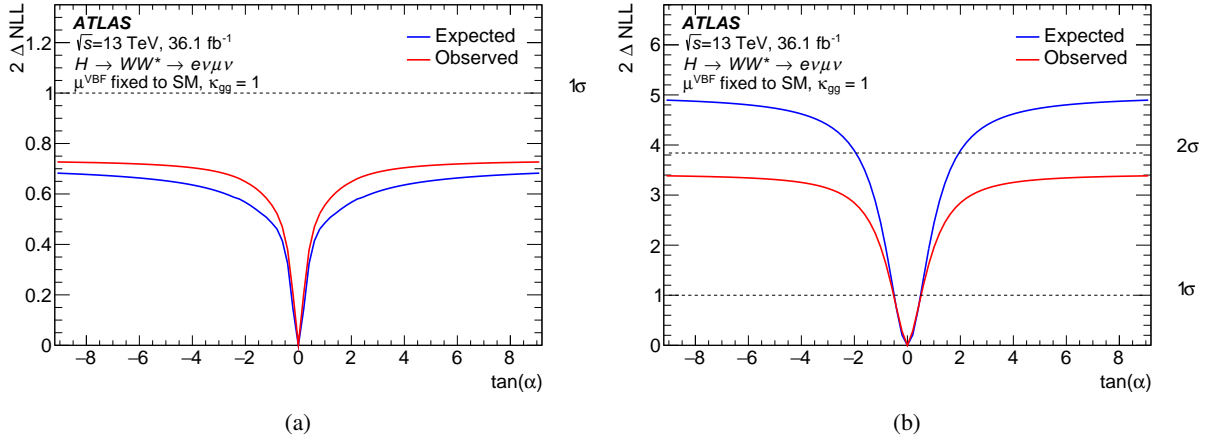
Figure 5: Expected and observed likelihood curves for scans (a) over \tan(\alpha) where only the shape is taken into account in the fit, and (b) over \tan(\alpha) when both shape and normalisation are used.
