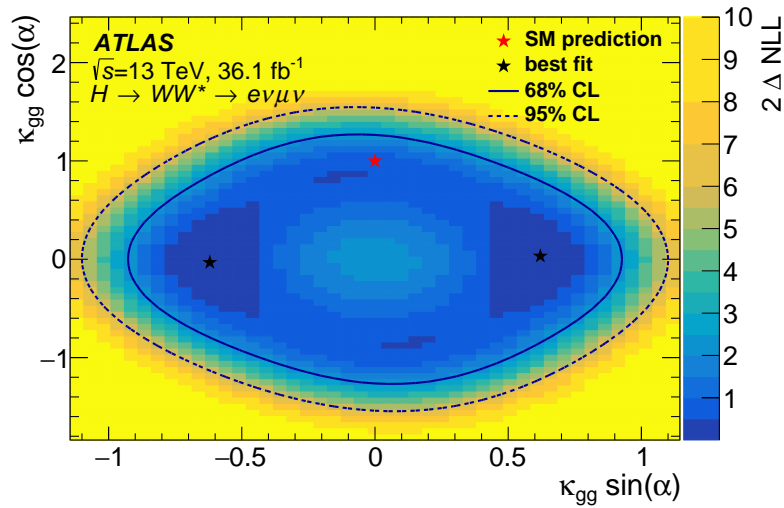
Figure 6: 68% and 95% CL two-dimensional likelihood contours of the CP-even and CP-odd coupling parameters \kappa_{gg} \cos(\alpha) and \kappa_{gg} \sin(\alpha) . The minima are represented by black stars, while the SM point is shown as a red star.
