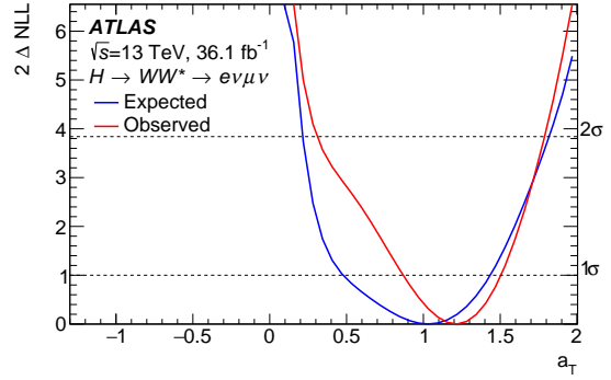
(b) a_T shape+rate fit with a_L = 1
