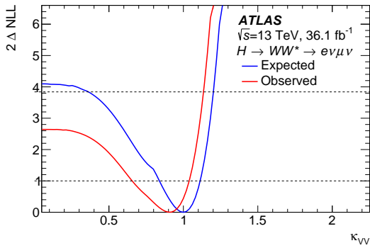
(a) \kappa_{VV} shape+rate fit with profiled \varepsilon_{VV}
