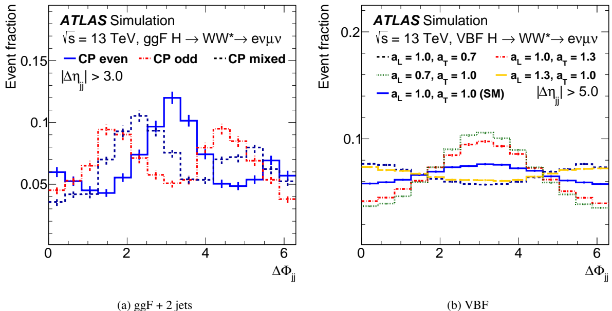
Figure 2: Distributions of the signed \Delta\Phi_{jj} observable shown for (a) CP-even, CP-odd and CP-mixed benchmark models of the ggF + 2 jets production mode, and (b) various configurations of the a_L and a_T parameters in VBF events. These comparisons are performed at the generator level using the predictions of the MADGRAPH5_aMC@NLO 2.4.2 + PYTHIA 8.212 [32] generators.
