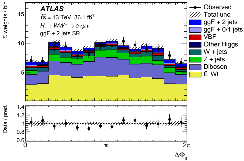
Figure 4: The weighted \Delta\Phi_{jj} post-fit distribution in the ggF + 2 jets signal region, with signal and background yields fixed from the fit to \tan(\alpha) using shape and rate information. Data-to-simulation ratios are shown at the bottom of the plot. The shaded areas depict the total uncertainty.
