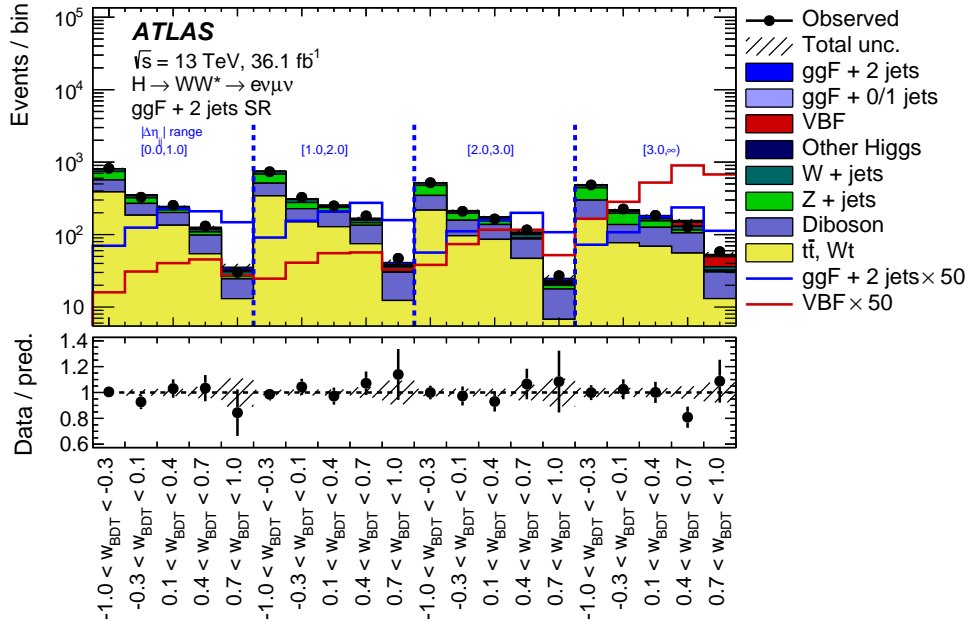
Figure 3: Post-fit distribution of the BDT response observable presented in the four |\Delta\eta_{jj}| categories of the ggF + 2 jets signal region, with signal and background yields fixed from the fit for \mu^{\text{ggF}+2\text{jets}} . Data-to-simulation ratios are shown at the bottom of the plot. The shaded areas depict the total uncertainty. The distributions of the ggF + 2 jets and VBF processes are overlaid with their respective contributions multiplied by 50.
