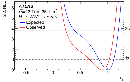
(c) a_L shape+rate fit with a_T = 1
