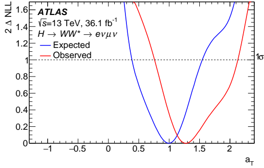
(a) a_T shape-only fit with a_L = 1
