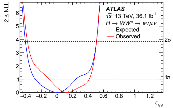
(b) \varepsilon_{VV} shape+rate fit with profiled \kappa_{VV}
