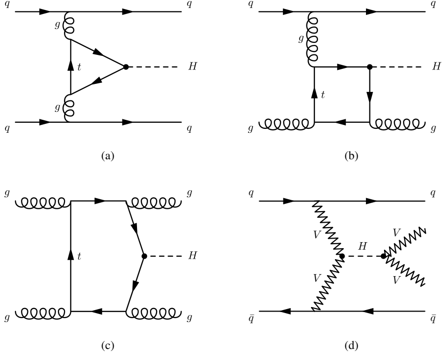
Figure 1: Examples of Feynman diagrams contributing to the production of a Higgs boson in association with two jets via the fusion of two gluons or two vector bosons at leading order in QCD. The presented diagrams show examples for the subprocesses (a) qq \rightarrow Hqq , (b) qg \rightarrow Hqg and (c) gg \rightarrow Hgg , as well as (d) the vector-boson fusion process and the subsequent decay of the Higgs boson into two vector bosons.
