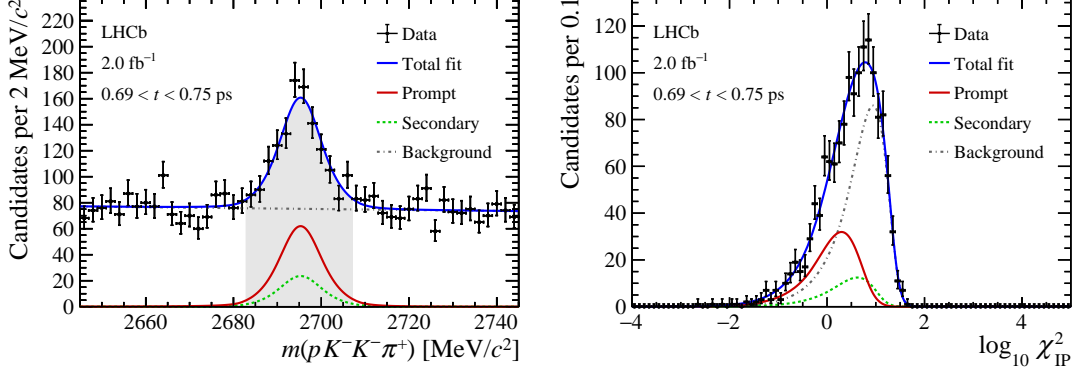
Figure 1: Distributions of (left) invariant mass and (right) \log_{10} \chi_{\text{IP}}^2 in the reduced mass region of [2683, 2707] \text{ MeV}/c^2 for the \Omega_c^0 data sample collected in 2018 in the decay-time interval of [0.69, 0.75] \text{ ps} , along with the fit results. The contributions of the signal, the secondary decays, and the combinatorial background are shown in red (solid), green (dashed), and gray (dash-dotted), respectively.
