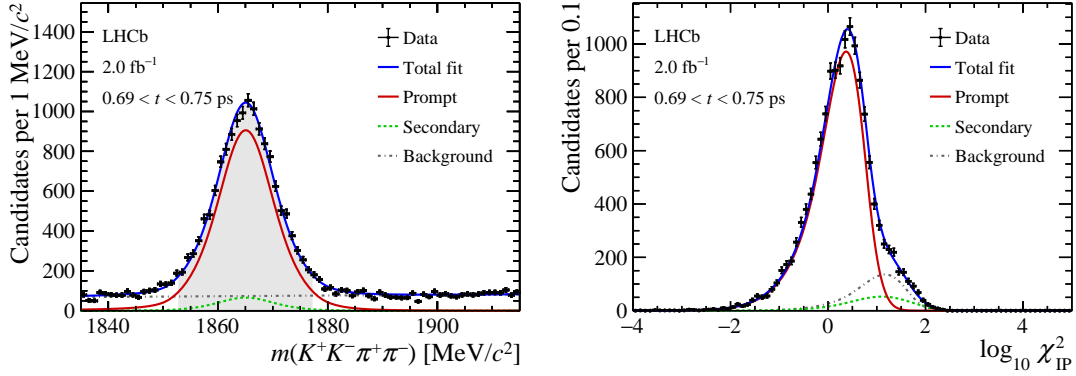
Figure 3: Distributions of (left) invariant mass and (right) \log_{10} \chi_{\text{IP}}^2 in the reduced mass region of [1853, 1877] MeV/ c^2 for the D^0 data sample collected in 2018 in the decay-time interval of [0.69, 0.75] ps, along with the fit results. The contributions of the signal, the secondary decays, and the combinatorial background are shown in red (solid), green (dashed), and gray (dash-dotted), respectively.
