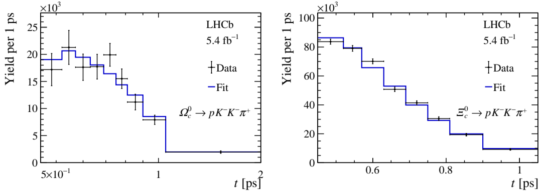
Figure 4: Decay-time distributions for the (left) \Omega_c^0 mode and the (right) \Xi_c^0 mode with the \chi^2 fit superimposed. The uncertainty on the data distribution is statistical only.
