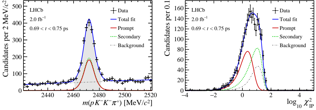
Figure 2: Distributions of (left) invariant mass and (right) \log_{10} \chi_{\text{IP}}^2 in the reduced mass region of [2461, 2481] \text{ MeV}/c^2 for the \Xi_c^0 data sample collected in 2018 in the decay-time interval of [0.69, 0.75] \text{ ps} , along with the fit results. The contributions of the signal, the secondary decays, and the combinatorial background are shown in red (solid), green (dashed), and gray (dash-dotted), respectively.
