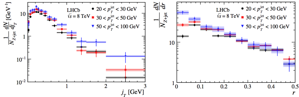
Figure 2: Measured j_T distributions (left) and r distributions (right) at \sqrt{s}=8 TeV [8].
