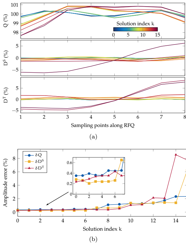
FIG. 10. Predicted field components (a) after applying the tuner adjustments yielded during tuning step 1 by discarding the smallest k singular values from the response matrix. Corresponding field component errors are reported in (b).
