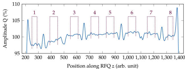
FIG. 6. Example measurement of Q component before tuning. Brackets visualize the windows over which the measurement is averaged to obtain the discrete sampling points.
