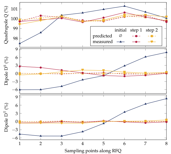
FIG. 11. Field components for nominal tuner position (initial) and after the first and second tuning step. Dashed lines indicate the field predicted by Eq. (14), while solid lines report the actually measured field.
