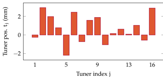
FIG. 13. Tuner positions after the final tuning step. A positive (negative) value indicates that the tuner was retracted (inserted) with respect to the nominal position.
