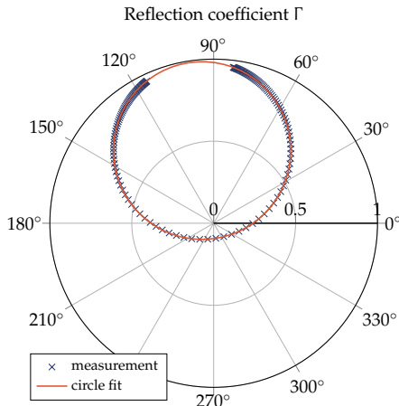
FIG. 15. Smith chart of the reflection coefficient \Gamma measured over a span of 1 MHz and the fitted circle. Only every tenth measurement point is shown for clarity.
