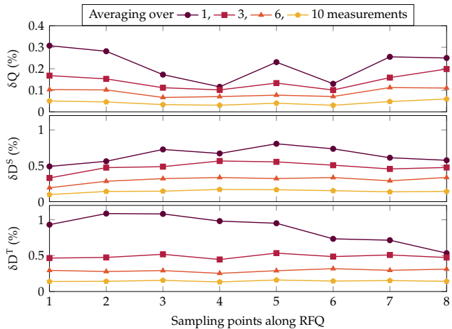
FIG. 7. Reduction of error in quadrupole component ( \delta Q ) and dipole components ( \delta D^S, \delta D^T ) when averaging over three, six, and ten measurements, compared to no averaging (one measurement). The source data was obtained from thirteen measurements carried out over several days.
