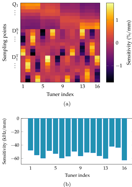
FIG. 9. Visual representation of response matrix \mathbf{R} except for the last row and column (a). Each entry represents the sensitivity of the Q (upper third), D^S (middle third), or D^T component (lower third) at one sampling point with respect to the tuner movement given in units of \%/mm (without normalization). The responses of the TE_{210} eigenfrequency to the movement of each tuner, i.e. the last row of \mathbf{R} , is shown in (b). A negative derivative means that the frequency is lowered when the tuner is retracted, as the total cavity inductance is increased.
