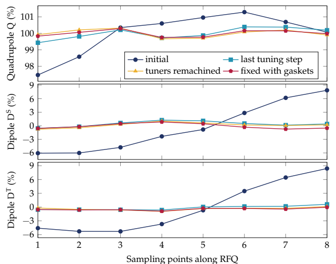
FIG. 14. Measured field components before tuning, after tuning, with remachined tuners, and for the final installation of the tuners with copper gaskets.
