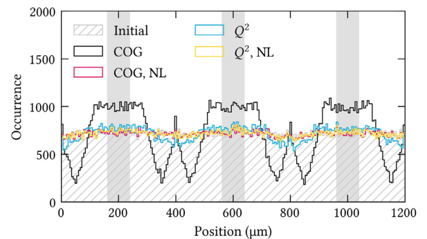
Fig. 14. Simulated position distributions for the different reconstruction methods and comparison with the initial position distribution.
