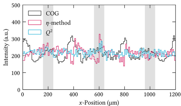
Fig. 13. Position distribution for the data from the test beam tracker. The neighbouring-logic was not available for these measurements, as they were performed with a different readout ASIC.
