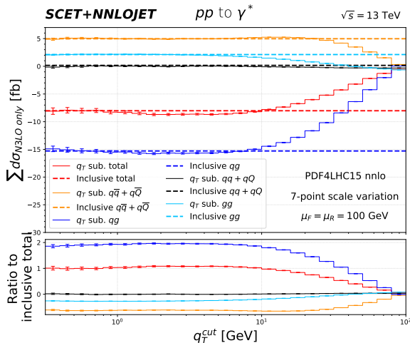
FIG. 2: Inclusive N 3 LO QCD corrections to total cross section for Drell-Yan production through a virtual photon. In the bottom panel we plot the ratio to the analytic calculation in [14].
