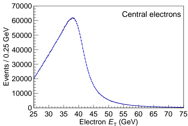
FIG. 6. Background-subtracted E_T distribution for electron candidates in the central region. The crosses are the data and the solid histogram is the simulation. The comparison between the data and the simulation yields a \chi^2 of 373 per 200 bins.
