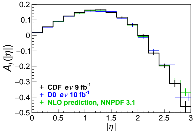
FIG. 26. Distributions of A_\ell(|\eta|) as a function of |\eta| for the Tevatron measurements previously shown in Fig. 25, along with the NLO prediction with NNPDF 3.1 PDFs. The bold (black) histogram is the result of this measurement and the (blue) crosses the D0 measurement [8]. The thin (green) histogram is the NLO prediction using the NNPDF 3.1 PDFs.
