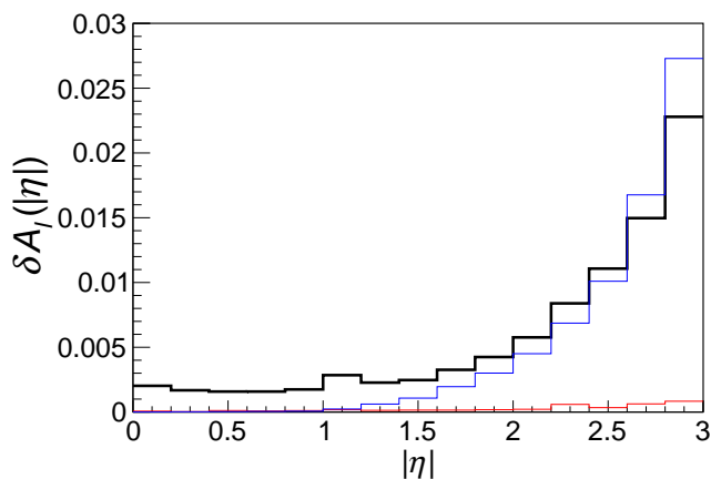
FIG. 24. \delta A_\ell(|\eta|) as a function of |\eta| , where \delta A_\ell denotes the data, PDF, or non-PDF uncertainty. The bold (black) histogram shows the statistical uncertainties of the data. The lowest (red) histogram is from the quadrature sum of the non-PDF systematic uncertainties. The remaining lighter-shaded (blue) histogram is the uncertainty due to PDFs. All uncertainties are bin-by-bin. The data and PDF uncertainties are taken from the diagonal terms of their respective covariance matrices.
