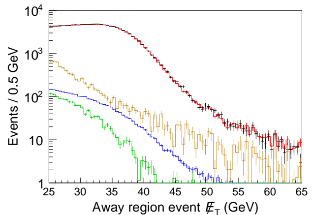
FIG. 14. \cancel{E}_T distributions for electron candidates in the plug calorimeter from the high-luminosity period, with n_{\text{vtx}} = 2 , and in the away region. The (black) crosses are the data and the (red) histogram overlapping the data is the simulation with all backgrounds. The backgrounds shown as examples from top to bottom are QCD (brown), \gamma^*/Z \rightarrow ee (blue), and W \rightarrow \tau\nu (green).
