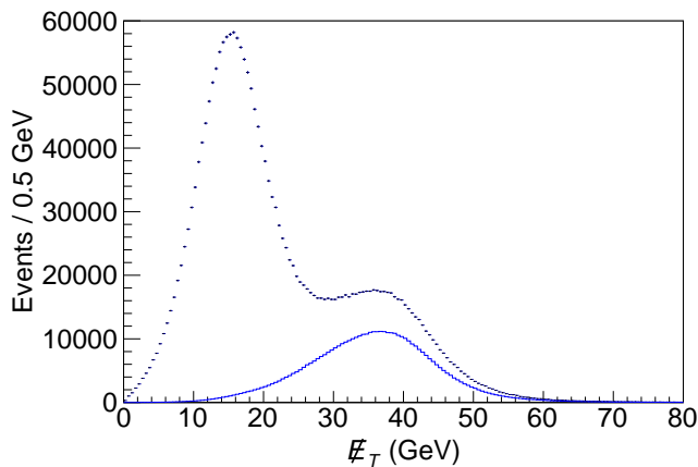
FIG. 32. E_T distribution for plug-region electrons rejected by the additional selection criteria. The (black) crosses are the data, and the (blue) histogram is the simulation, which contains about 18% of the events without the additional requirements. The online-trigger selection allows the peak at low values of E_T .
