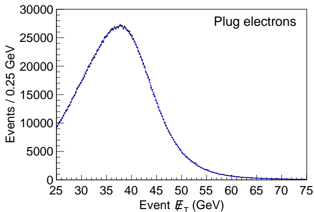
FIG. 11. Background-subtracted E_T distribution for electron candidates in the plug region. The crosses are the data and the solid histogram is the simulation. The comparison between the data and the simulation yields a \chi^2 of 310 per 200 bins.
