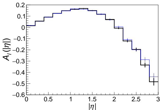
FIG. 22. Observed lepton asymmetry A_\ell(|\eta|) as a function of |\eta| . The bold (black) histogram is the measurement in the \eta \geq 0 region, and the lighter (blue) histogram is in the \eta < 0 region. The measurements include all corrections, and the uncertainties are statistical only, and evaluated bin-by-bin. Bin-centering corrections are not a part of the measurements.
