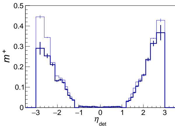
FIG. 20. Charge-misidentification rates m^+ averaged over the sectors of a ring, versus \eta_{\text{det}} . The bold (black) histogram is for the data, and the lighter (blue) histogram for the simulation.
