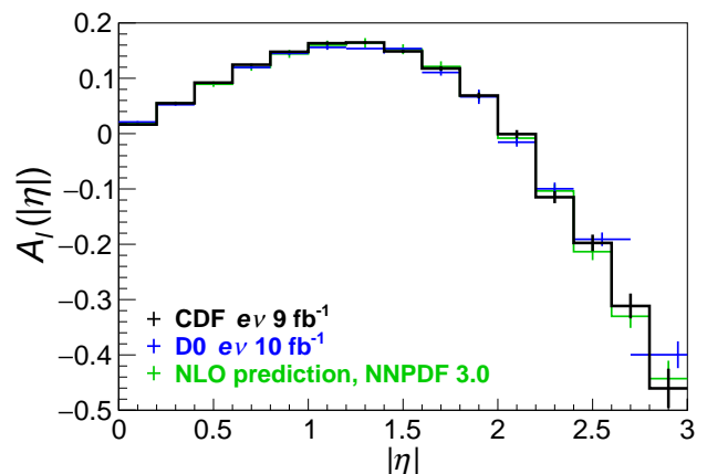
FIG. 25. CP-folded distributions of A_\ell(|\eta|) as a function of |\eta| . The bold (black) histogram is the result of this measurement, and the uncertainties shown are evaluated bin-by-bin and include both statistical and systematic contributions. The (blue) crosses represent the measurement from D0 [8]. For D0, the bin size is also 0.2 |\eta| -units wide, except for these regions: 1.2–1.6, 2.4–2.7, and 2.7–3.2. Both the CDF and D0 measurements use all the data from Run II of the Tevatron Collider. The thin (green) histogram is the NLO prediction using the NNPDF 3.0 PDFs.
