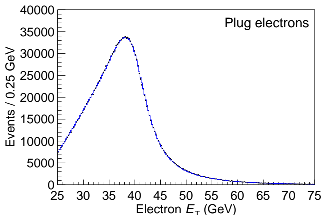
FIG. 7. Background-subtracted E_T distribution for electron candidates in the plug region. The crosses are the data and the solid histogram is the simulation. The comparison between the data and the simulation yields a \chi^2 of 317 per 200 bins.
