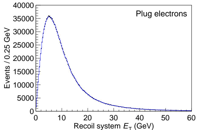
FIG. 9. Background-subtracted E_T^{X(\text{obs})} distribution for electron candidates in the plug region. The crosses are the data and the solid histogram is the simulation. The comparison between the data and the simulation yields a \chi^2 of 402 per 240 bins.
