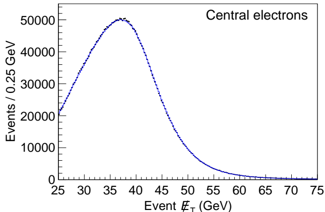
FIG. 10. Background-subtracted E_T distribution for electron candidates in the central region. The crosses are the data and the solid histogram is the simulation. The comparison between the data and the simulation yields a \chi^2 of 260 per 200 bins.
