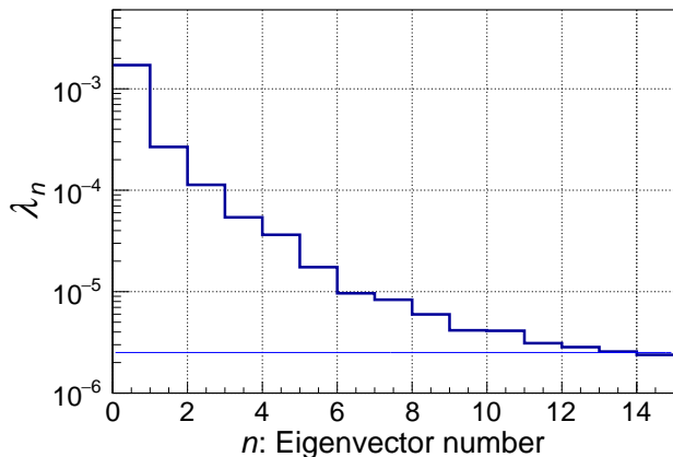
FIG. 27. Eigenvalues \lambda_n as a function of the eigenvector number n from the covariance matrix of the asymmetry measurement. The bold (black) histogram shows the eigenvalues, and the lighter (blue) horizontal line corresponds to the smallest value of the diagonal terms of the covariance matrix.
