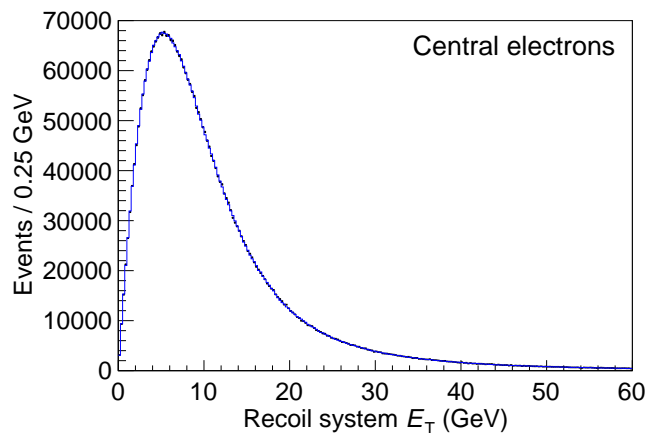
FIG. 8. Background-subtracted E_T^{X(\text{obs})} distribution for electron candidates in the central region. The crosses are the data and the solid histogram is the simulation. The comparison between the data and the simulation yields a \chi^2 of 256 per 240 bins.
