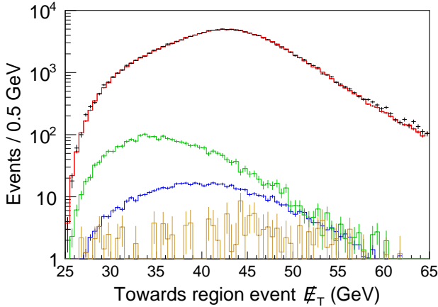
FIG. 16. E_T distributions for electron candidates in the plug calorimeter from the high-luminosity period, with n_{\text{vtx}} = 2 , and in the towards region. The (black) crosses are the data and the (red) histogram overlapping the data is the simulation with all backgrounds. The backgrounds shown as examples from top to bottom are W \rightarrow \tau\nu (green), \gamma^*/Z \rightarrow ee (blue), and QCD (brown).
