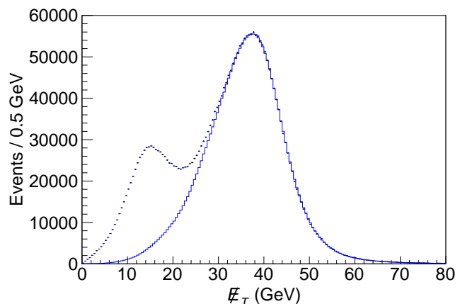
FIG. 31. \cancel{E}_T distribution for plug-region electrons accepted by the additional selection criteria. The (black) crosses are the data, and the (blue) histogram is the simulation. The online-trigger selection allows the peak at low values of \cancel{E}_T .
