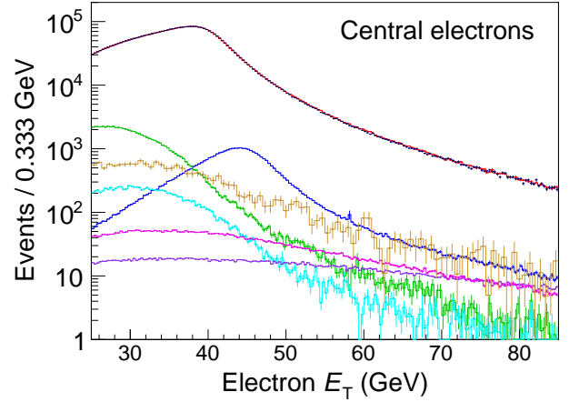
FIG. 17. E_T distributions of central-region electrons. The data are the crosses (black) and the simulation with all backgrounds is the histogram (red) overlapping the data. The individual backgrounds are the lower histograms, and from the top to bottom along the left edge of the plot they are the W \rightarrow \tau\nu (green), QCD (brown), \gamma^*/Z \rightarrow \tau^+\tau^- (cyan), \gamma^*/Z \rightarrow ee (blue), diboson (magenta), and t\bar{t} (purple) contributions.
