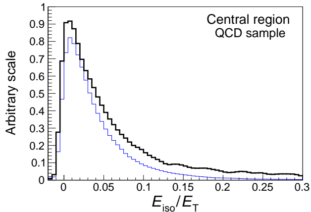
FIG. 12. Shape of the E_{\text{iso}}/E_T distribution of central-region events from the QCD sample. The bold (black) histogram is the data and the lighter (blue) histogram is the expected contribution of the non-QCD processes.
