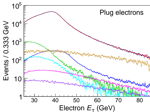
FIG. 18. E_T distributions of plug-region electrons. The data are the crosses (black) and the simulation with all backgrounds is the histogram (red) overlapping the data. The individual backgrounds are the lower histograms, and from the top to bottom along the left edge of the plot they are the W \rightarrow \tau\nu (green), QCD (brown), \gamma^*/Z \rightarrow ee (blue), which peaks around 40 GeV, \gamma^*/Z \rightarrow \tau^+\tau^- (cyan), diboson (magenta), and t\bar{t} (purple) contributions.
