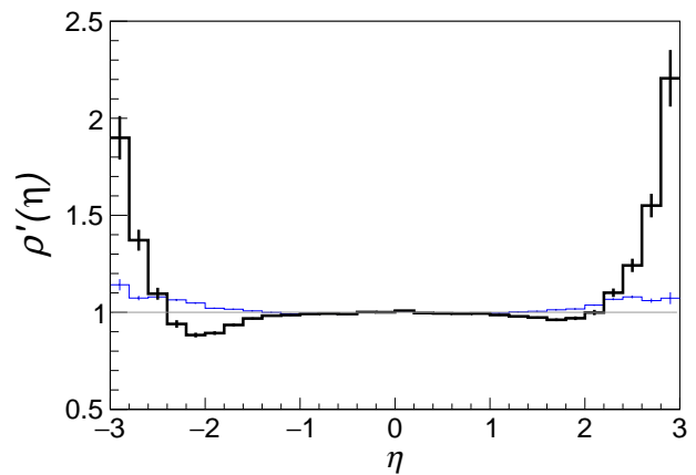
FIG. 21. Dependence of \rho'(\eta) on \eta . The bold (black) histogram includes the accounting of charge misidentification while the lighter (blue) histogram does not. The uncertainties shown are statistical and are evaluated bin-by-bin. The horizontal (gray) line is a unit-value reference.
