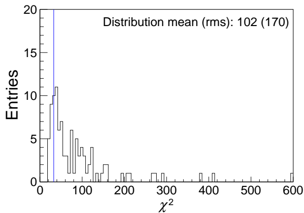
FIG. 29. Distribution of \chi^2 values from the comparisons between the measurement and the individual predictions over 15 bins for the NNPDF 3.0 ensemble of PDFs. The light (blue) vertical line on the plot shows the \chi^2 value (32.6) of the ensemble-averaged prediction. One of the ensemble PDFs gives a \chi^2 value of 1548, and is not shown.
