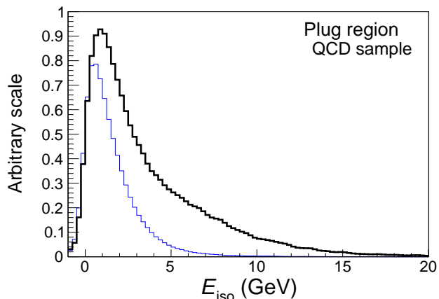
FIG. 13. Shape of the E_{\text{iso}} distribution of plug-region events from the QCD sample. The bold (black) histogram is the data and the lighter (blue) histogram is the expected contribution of the non-QCD processes.
