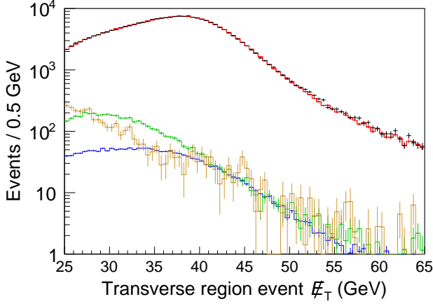
FIG. 15. E_T distributions for electron candidates in the plug calorimeter from the high-luminosity period, with n_{\text{vtx}} = 2 , and in the transverse region. The (black) crosses are the data and the (red) histogram overlapping the data is simulation with all backgrounds. The backgrounds shown as examples from top to bottom along the y axis are QCD (brown), W \rightarrow \tau\nu (green), and \gamma^*/Z \rightarrow ee (blue).
