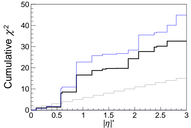
FIG. 28. Cumulative \chi^2 as a function of |\eta|' . The bold (black) [light (blue)] histogram is for NNPDF 3.0 [3.1]. The lowermost (gray) histogram is for an ideal 15-bin measurement and a prediction whose underlying physics matches that of the measurement. Differences between the underlying PDFs of the data and that of the calculation result in differences between the ideal and observed \chi^2 distributions.
