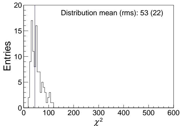
FIG. 30. Distribution of \chi^2 values from the comparisons between the measurement and the individual predictions over 15 bins for the NNPDF 3.1 ensemble of PDFs. The light (blue) vertical line on the plot shows the \chi^2 value (44.9) of the ensemble-averaged prediction. All \chi^2 values are contained within the plot.
