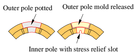
Fig. 6. TQC coil styles
