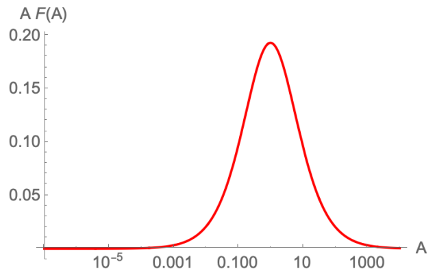
FIG. 1: The function A\mathcal{F}(A) defined in (40) that sets the scale of the backreaction.
