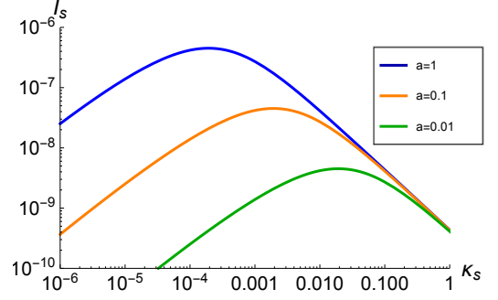
FIG. 3: The integral I_s in (59) determines in units of \Omega_D \bar{\varepsilon} H the relative size of backreaction for a dark matter component with sound velocity c_s^2 = \kappa_s a^{\nu_s - 1} . The plot is for \nu_s = 1 .
