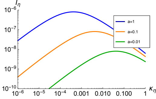
FIG. 2: The integral I_\eta in (56) determines the relative size of backreaction for a viscous dark matter component in units of \Omega_D \bar{\varepsilon} H . The plot is obtained for c_\eta^2 = \kappa_\eta a^{\nu_\eta - 1} with \nu_\eta = 1 .
