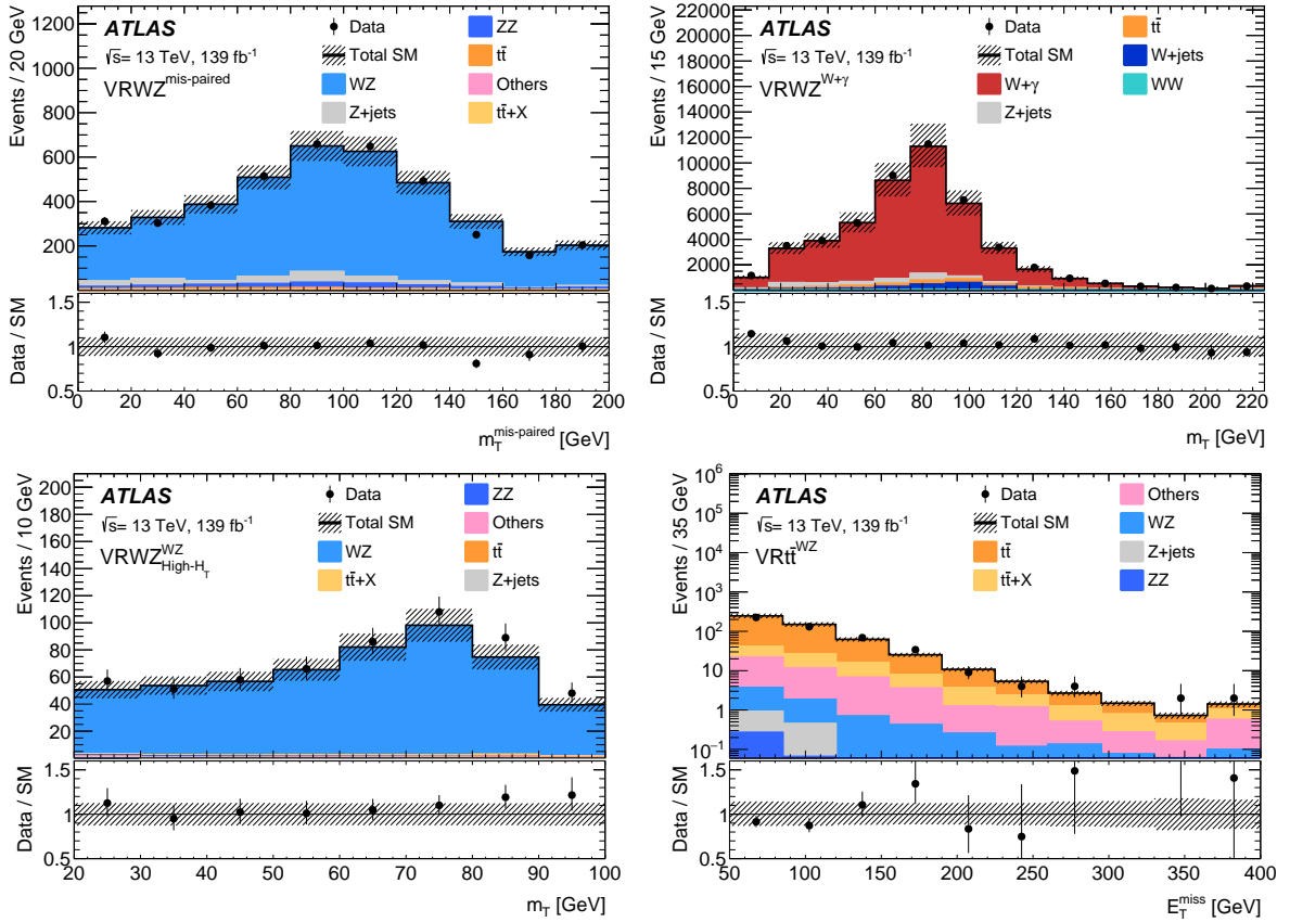
Figure 3: Distributions of m_T showing the data and the pre-fit expected background in (top left) the mis-paired lepton validation region and (top right) the W+ \gamma validation region, used to validate the WZ background. Distributions of (bottom left) m_T in VRWZ ^{\text{high-H}_T} and (bottom right) E_T^{\text{miss}} in VR t\bar{t}^{\text{WZ}} , showing the data and the post-fit expected background in each region. The last bin includes overflow. The ‘Others’ category contains backgrounds from single-top, WW, triboson, Higgs and rare top processes. The bottom panel shows the ratio of the observed data to the predicted yields. The hatched bands indicate the combined theoretical, experimental, and MC statistical uncertainties.
