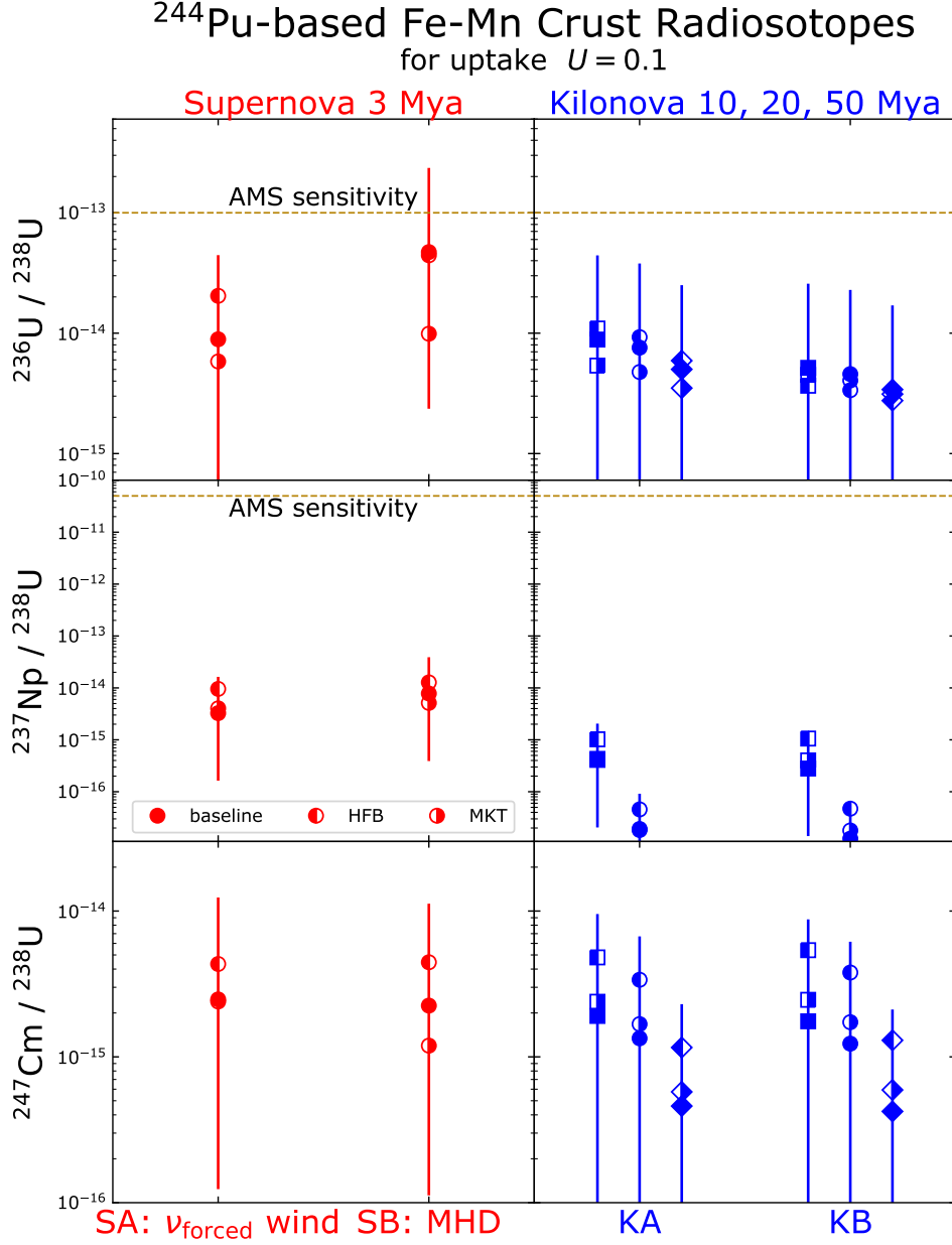
Figure 13. Predicted abundances of the actinides ^{236}\text{U} , ^{237}\text{Np} , and ^{247}\text{Cm} in Fe-Mn crusts, shown for the same SN and KN models as in Fig. 12. We use ^{238}\text{U} as the reference standard for all three species. The results from our baseline calculations are shown as full symbols, and the half-filled symbols are results from HFB and MKT calculations.
