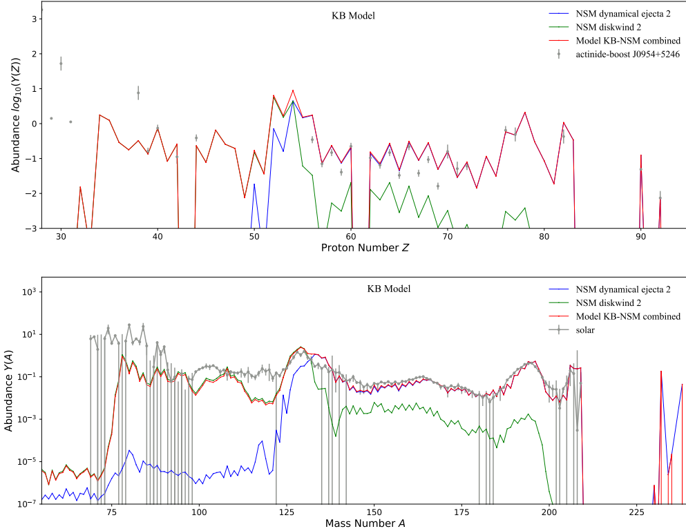
Figure 6. Upper panel: The abundances (at t \sim 10\text{Gyr} ) of r -process nuclei produced in simulations of KN more neutron-rich dynamical ejecta from Bovard et al. (2017) (blue) and of disk neutrino-driven wind from Just et al. (2015) (green), and a mixture (KB, red) fitted to the measurements of the actinide-boost star J0954+5346 ( Holmbeck et al. 2018 ), plotted as functions of the atomic number Z . Lower panel: The corresponding abundance pattern of model KB compared with solar abundance data ( Arnould et al. 2007 ), plotted as functions of the atomic weight A .
