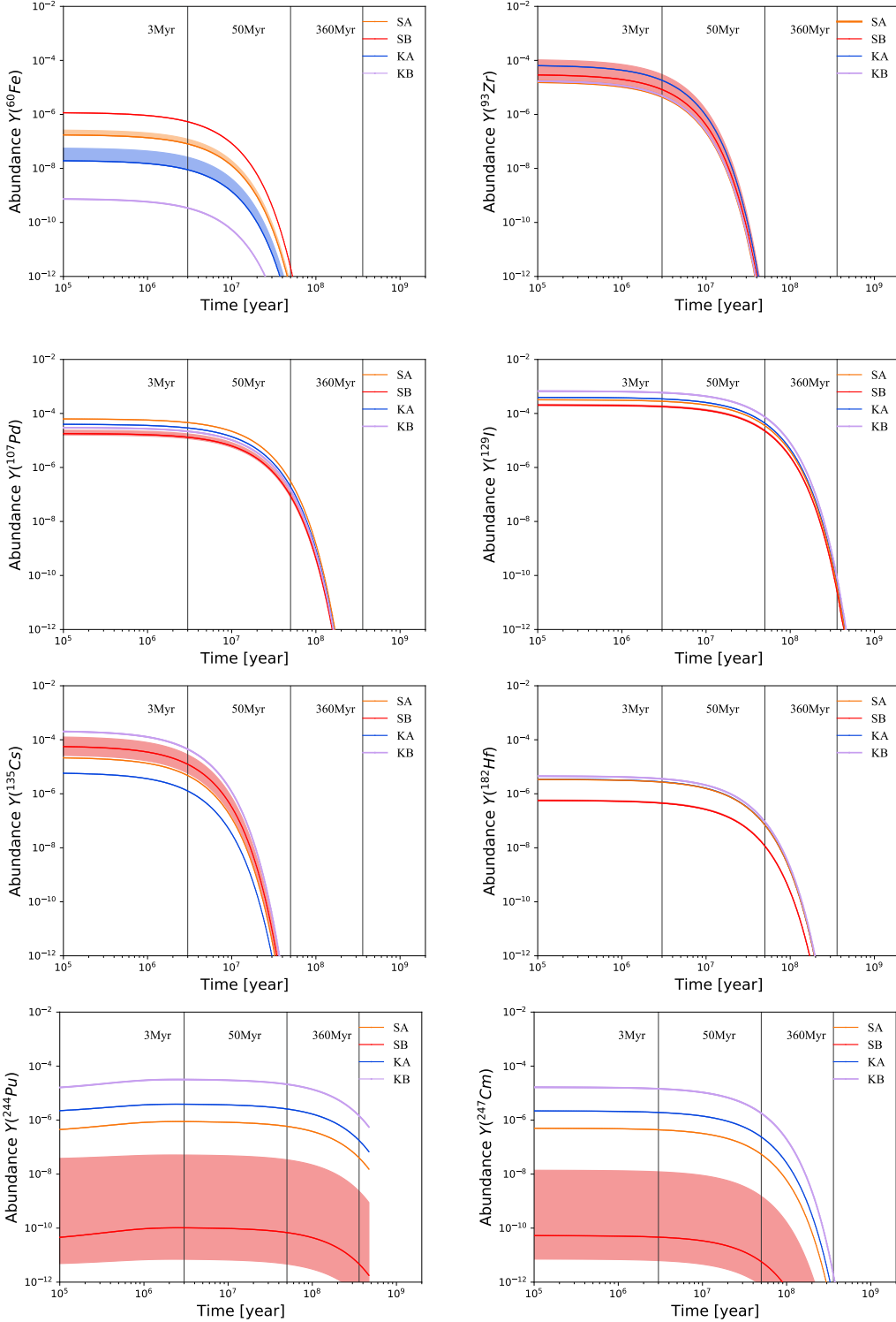
Figure 7. The time evolutions of the relative abundances of ^{60}\text{Fe} , ^{93}\text{Zr} , ^{107}\text{Pd} , ^{129}\text{I} , ^{135}\text{Cs} , ^{182}\text{Hf} , ^{244}\text{Pu} , and ^{247}\text{Cm} from an r -process event as calculated with the different astrophysical models described in Table 3, with the total mass of r -process species normalized to unity for each model. The solid lines were obtained using our baseline r -process calculation, and the shaded bands are the ranges due to uncertainties resulting from the adoption of different nuclear data (HFB masses from Goriely et al. (2009) or \beta -decay rates from Marketin et al. (2016) for both SN and KN models, or fission yields from Kodama & Takahashi (1975) for KN models, in addition to the baseline nuclear data) in this calculation (orange: SA; red: SB; blue: KA; and light purple: KB). The vertical lines indicate the age of the supernova explosion \sim 3 Mya attested by discoveries of deposits of ^{60}\text{Fe} , an age of 50 Mya comparable with the half-life of ^{244}\text{Pu} , and the age of the end-Devonian extinction(s) \sim 360 Mya.
