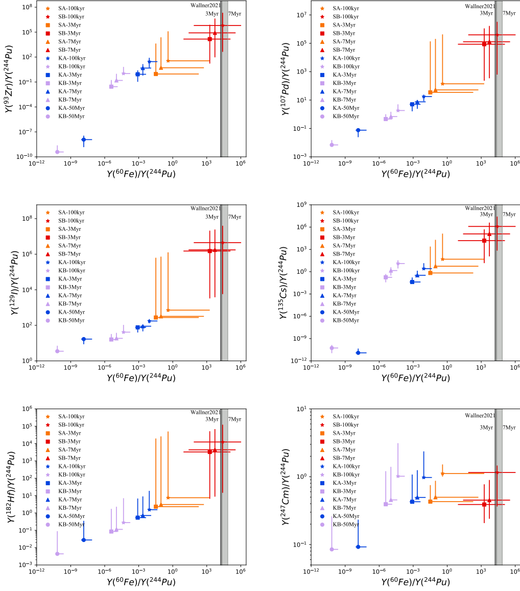
Figure 10. Scatterplots of the isotope abundance ratios of ^{93}\text{Zr} , ^{107}\text{Pd} , ^{129}\text{I} , ^{135}\text{Cs} , ^{182}\text{Hf} , and ^{247}\text{Cm}/^{244}\text{Pu} versus ^{60}\text{Fe}/^{244}\text{Pu} after times 100 kyr, 3 Myr and 7 Myr (also 50 Myr for the KN models KA and KB), as calculated with the different astrophysical r-process models described in Table 3. The points are the isotope ratios obtained from the baseline r-process calculations, and the error bars denote the variations due to the different sets of nuclear models (HFB masses from Goriely et al. (2009) or \beta -decay rates from Marketin et al. (2016) for both SN and KN models, in addition to the baseline nuclear data) adopted in the r-process. Note that the isotope ratios presented here are only from the r-process nucleosynthesis. For SNe, ^{60}\text{Fe} is mainly produced in the pre-SN stage and through explosive nucleosynthesis; thus the isotope ratios of ^{60}\text{Fe}/^{244}\text{Pu} in the plot are actually the lower limit for SN models SA and SB. The shaded bands are the measured isotope ratios of ^{60}\text{Fe}/^{244}\text{Pu} at \sim 3 Myr (1.34-4.57 Myr; dark gray) and \sim 7 Myr (4.57-9.0 Myr; gray) time periods from Wallner et al. (2021).
