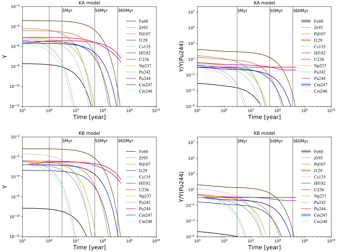
Figure 9. The time evolution of the abundances Y (left) and ratios Y/Y(^{244}\text{Pu}) (right) of r -process nuclei of interest from KM models KA (top) and KB (bottom). The vertical lines correspond to the age of the SN explosion \sim 3 Mya attested by discoveries of deposits of ^{60}\text{Fe} , \sim 50 Mya comparable with the half-life of ^{244}\text{Pu} , and the time since the end-Devonian extinction(s) \sim 360 Mya. The ratio ranges due to the nuclear variations as described in the text for ^{60}\text{Fe} , ^{129}\text{I} and ^{247}\text{Cm} to ^{244}\text{Pu} are shown in shaded bands of black, brown, and blue, respectively.
