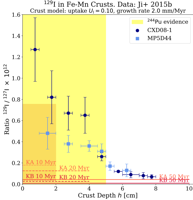
Figure 14. An example of the potential power of ^{129}\text{I} measurements. We show an estimate of the evolution with depth of the ^{129}\text{I}/^{127}\text{I} isotope ratio, based on the AMS data of Ji et al. (2015b). The horizontal lines represent the ratio ^{129}\text{I}/^{127}\text{I} that would be generated within the KA and KB models occurring at the indicated times t_{\text{KN}} in the past; these represent a floor below which the natural ^{129}\text{I} background cannot fall. The KA curves for t_{\text{KN}} = (10, 20) Myr are off-scale. These model lines assume a crust iodine uptake U_{\text{I}} = 0.1 and a constant growth rate \dot{h}_0 = 2 mm/Myr. Model uncertainties for t(\text{KB}) = 10 Myr are shown as a red band; similar ranges apply to the other cases. Model line heights scale as U_{\text{I}} \exp(-t_{\text{KN}}/\tau_{129}) , and maximum depth scales as h_{\text{max}} = \dot{h}_0 t_{\text{KN}} . The yellow band shows the extent of ^{244}\text{Pu} evidence using the assumed \dot{h}_0 .
