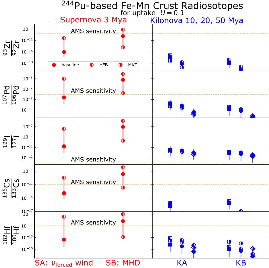
Figure 12. Radioisotope predictions normalized to the Wallner et al. (2015) ^{244}\text{Pu} flux from Eqs. (4) and (5). The predictions are normalized to a 10% uptake, and assume dust efficiency equal to that of Pu; for other values multiply by U_i f_i / f_{\text{Pu}} . The uncertainties are only those due to the ^{244}\text{Pu} flux, and the measurement limits are those listed in Table 9. The predictions are from (left panels) the SN r-process models after 3 Myr and (right panels) the KN r-process models after 10, 20, and 50 Myr. The results from our baseline calculations are shown as full symbols, and the half-filled symbols are results from HFB and MKT calculations. A minor change to the figure should be made for ^{93}\text{Zr}/^{92}\text{Zr} from 6 \times 10^{-11} to a new value of 2 \times 10^{-11} in light of a new citation that has been added to the text.
