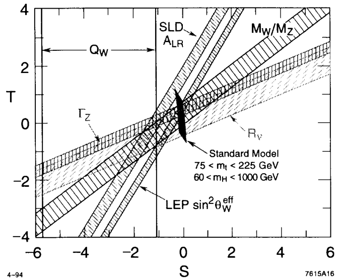
Figure 4: Constraints on S, T from electroweak data.
