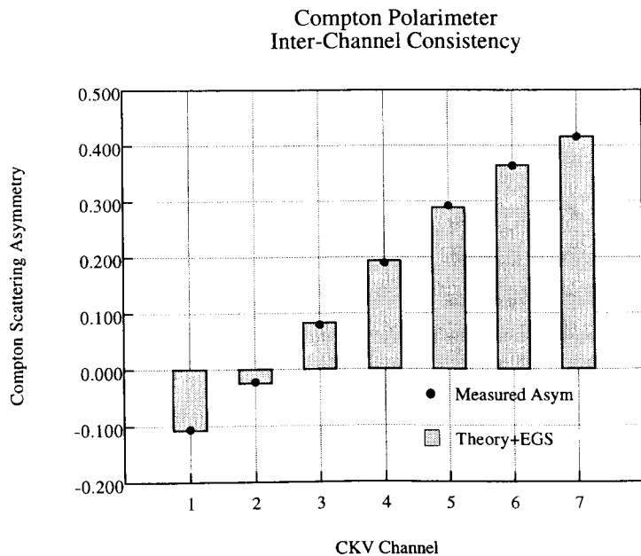
Figure 3: Measured and simulated Compton asymmetry.
