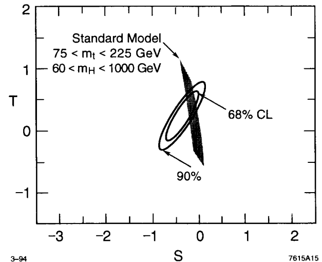
Figure 5: S, T fit to the world's electroweak data.
