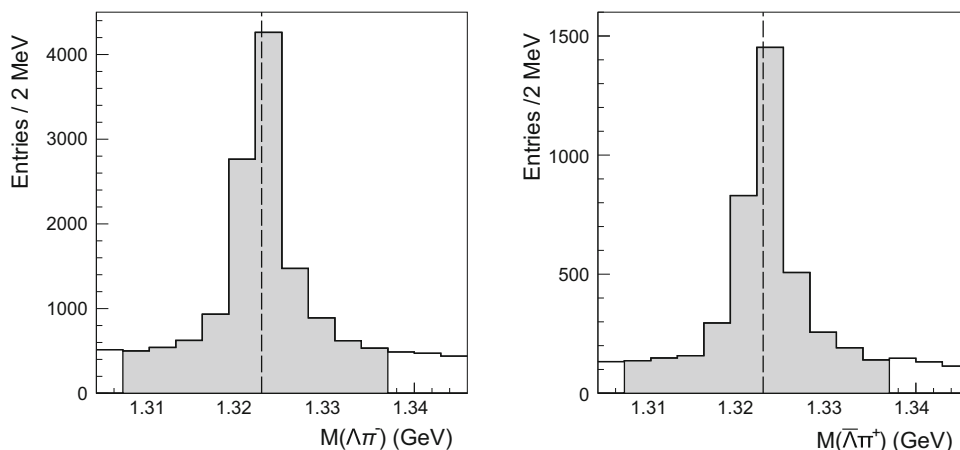
Fig. 3 The \Lambda \pi^- ( \bar{\Lambda} \pi^+ ) invariant mass spectrum of \Xi^- ( \bar{\Xi}^+ ) candidates are shown in the left panel (right panel). Filled areas indicate the mass range of the selected candidates. The vertical dashed black line shows the nominal PDG \Xi mass
